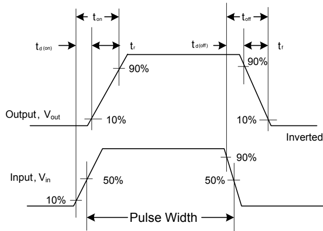
Figure 2. Switching Waveforms
