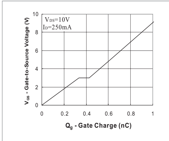
Fig.7 - Gate Charge
