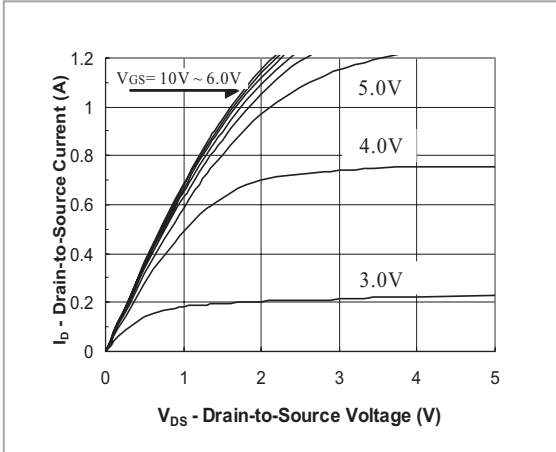
FIG.1- Output Characteristic
