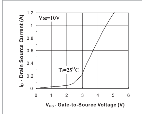
FIG.2- Transfer Characteristic
