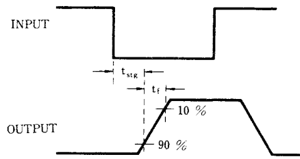
t off = t stg + t f
