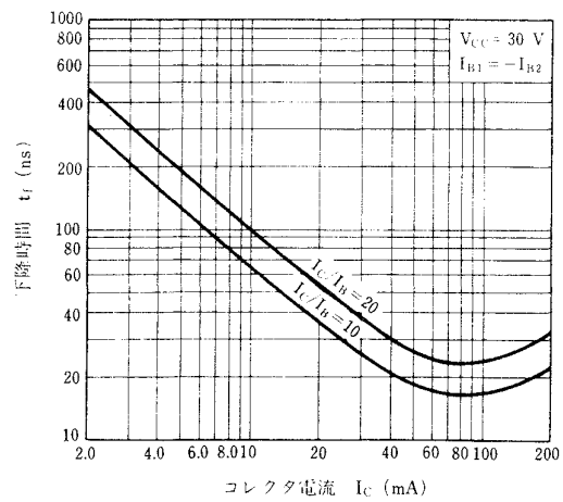
FALL TIME vs. COLLECTOR CURRENT
