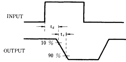
t on = t d + t r
