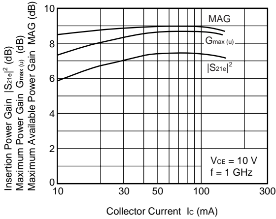
INSERTION POWER GAIN, MAXIMUM POWER GAIN, MAG vs. COLLECTOR CURRENT
