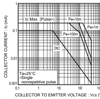
Fig.9 Safe operating area (2SC4505)
