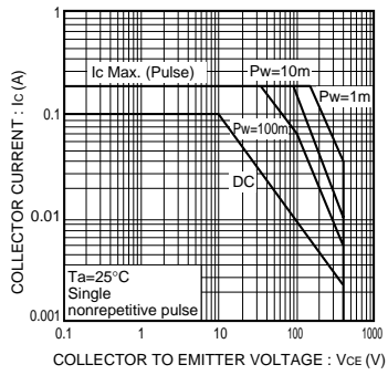
Fig.10 Safe operating area (2SC4620)
