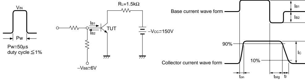
Fig.11 Switching time measurement circuit
