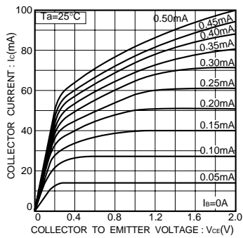
Fig.2 Grounded emitter output characteristics (1)
