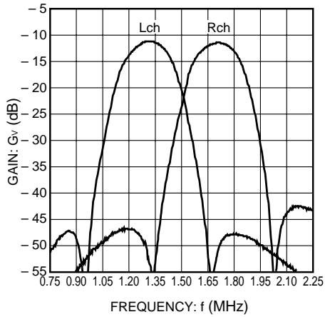
Fig. 3 FM BPF frequency characteristics (NTSC)
