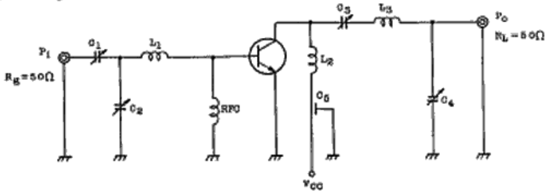
Fig. P 0 TEST CIRCUIT
