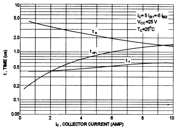
SWITCHING TIME
