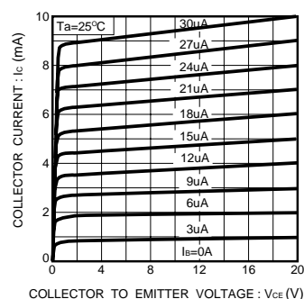
Fig.3 Grounded emitter output characteristics (2)
