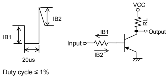
Figure 1 Switching Time Test Circuit & Timing Chart
