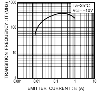
Fig.9 Transition Frequency
