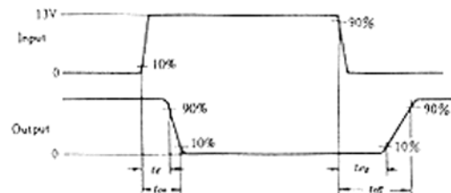
RESPONSE WAVEFORM
