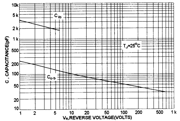
CAPACITANCE
