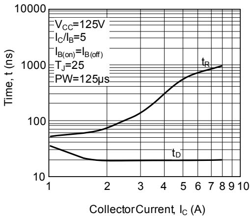
Figure 10. Turn-On Time(Resistive Load)
