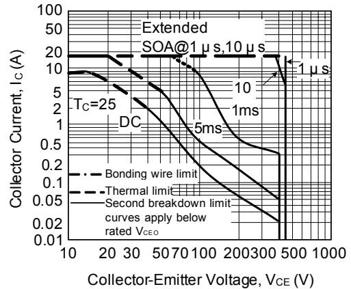
Figure 7. Maximum Forward Bias Safe Operating Area
