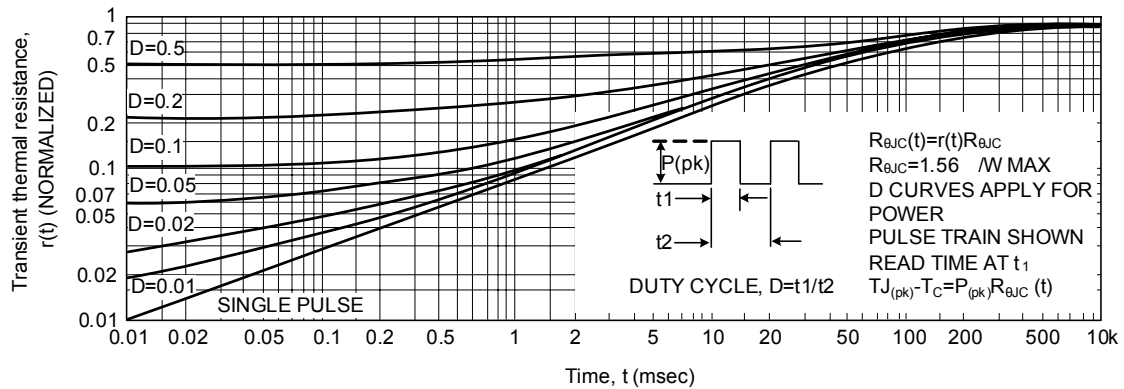
Figure1. Typical Thermal Response
