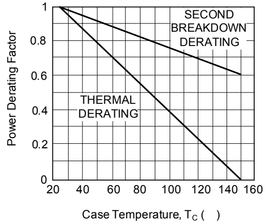
Figure 9. Forward Bias Power Derating
