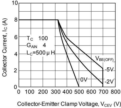
Figure 8. Maximum Reverse Bias Switching Safe Operating Area
