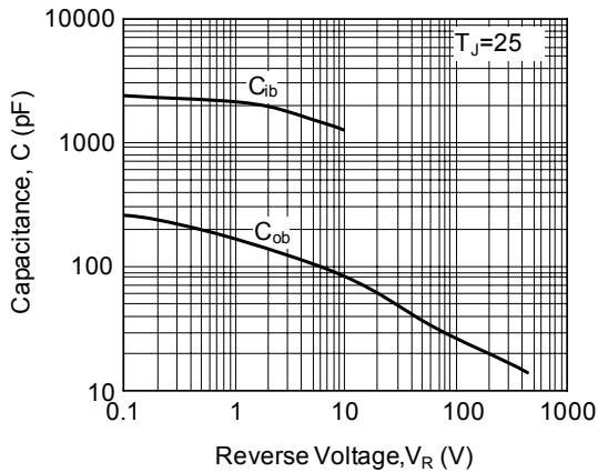
Figure 6. Capacitance
