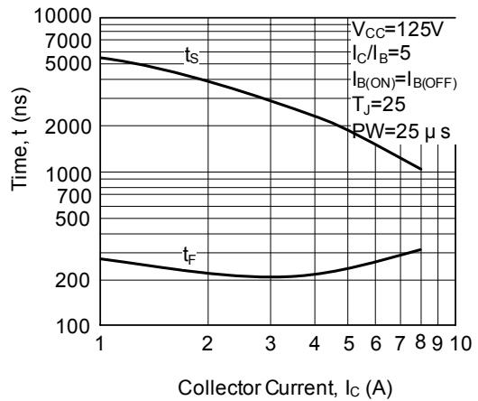
Figure 11. Turn-Off Time(Resistive Load)
