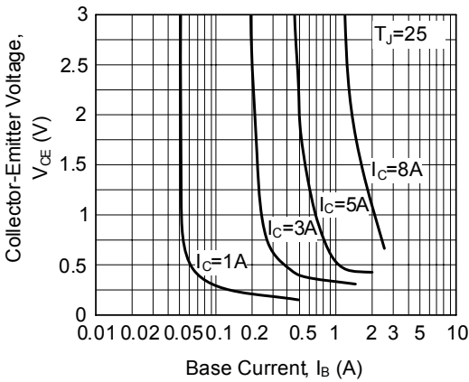
Figure 4. Collector Saturation Region
