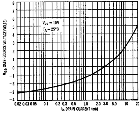
FIGURE 4 — 2N3797
