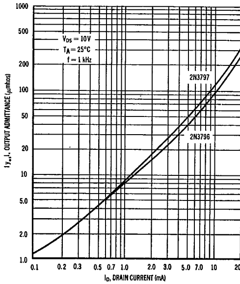
FIGURE 6 — OUTPUT ADMITTANCE
