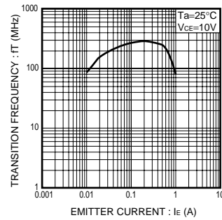
Fig.9 Transition Frequency : fT
