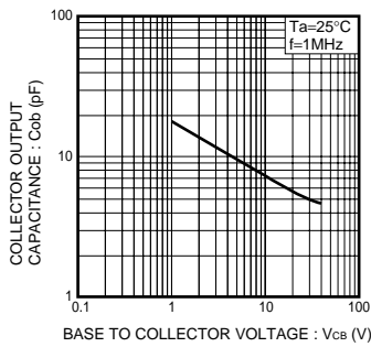
Fig.10 Collector Output Capacitance : Cob
