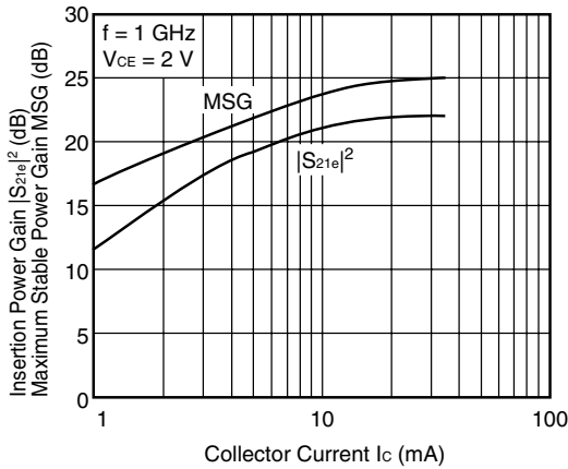
INSERTION POWER GAIN, MSG vs. COLLECTOR CURRENT
