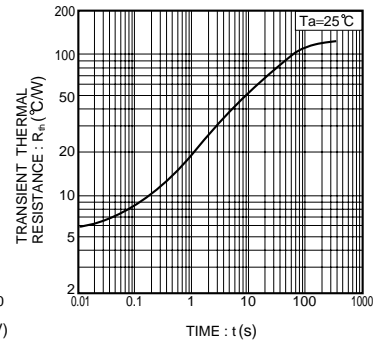
Fig.12 Transient thermal resistance (2SB1237)
