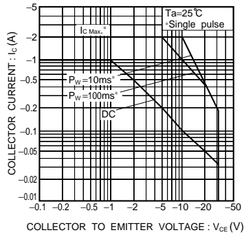
Fig.11 Safe operation area (2SB1237)
