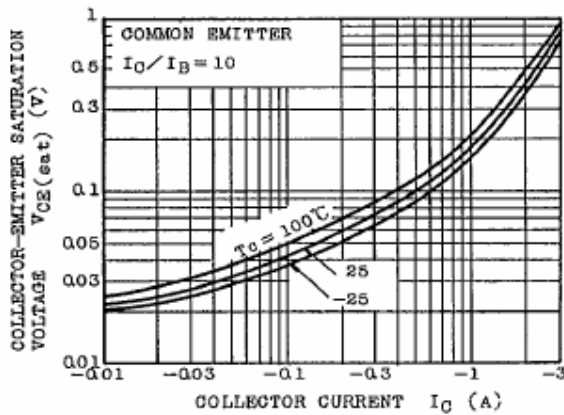
Fig.5 Collector-Emitter Saturation Voltage
