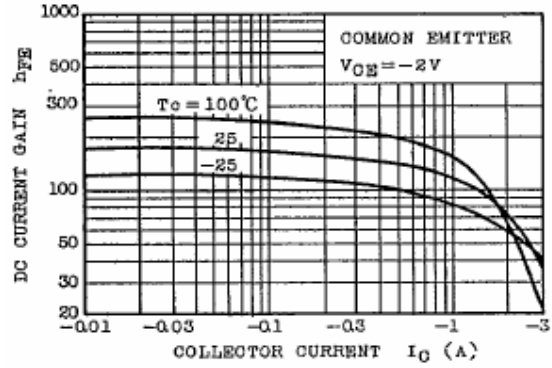
Fig.4 DC current Gain
