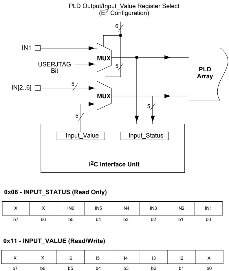
Figure 1-26. I 2 C Digital Input Interface
