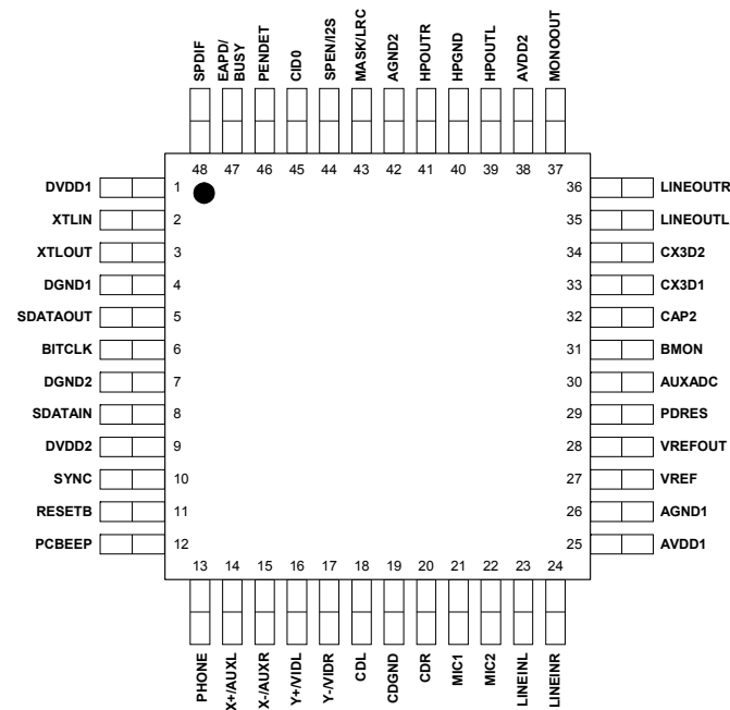
Figure 1 TQFP Pinout
