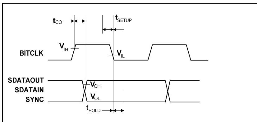
Figure 8 Data Setup and Hold (50pF External Load)
