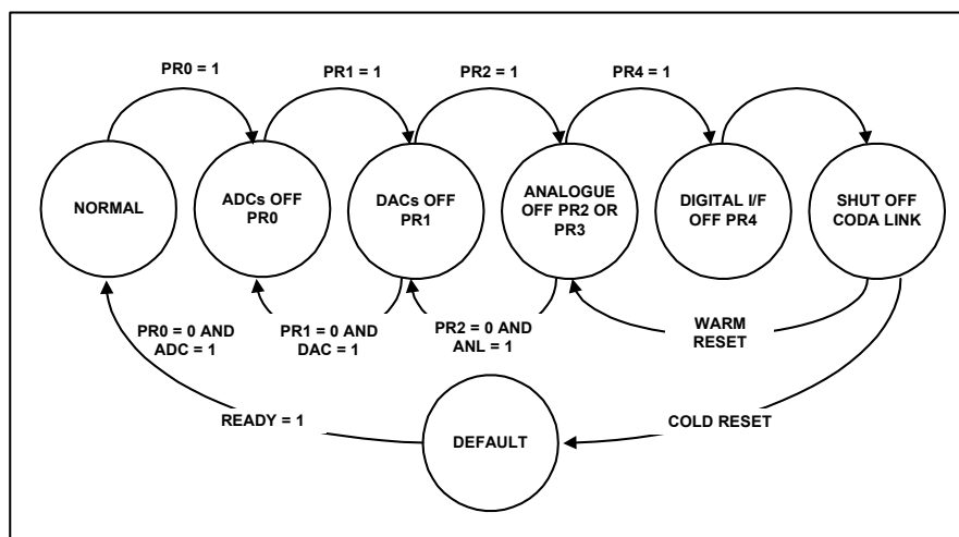
Figure 16 An Example of the WM9705 Powerdown/Powerup Flow
