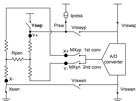
Figure 24 Pressure Measurement
