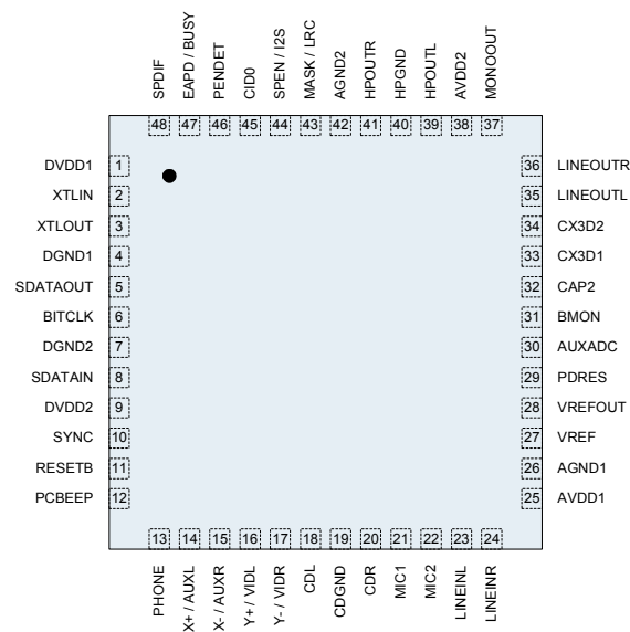
Figure 2 QFN Pinout
