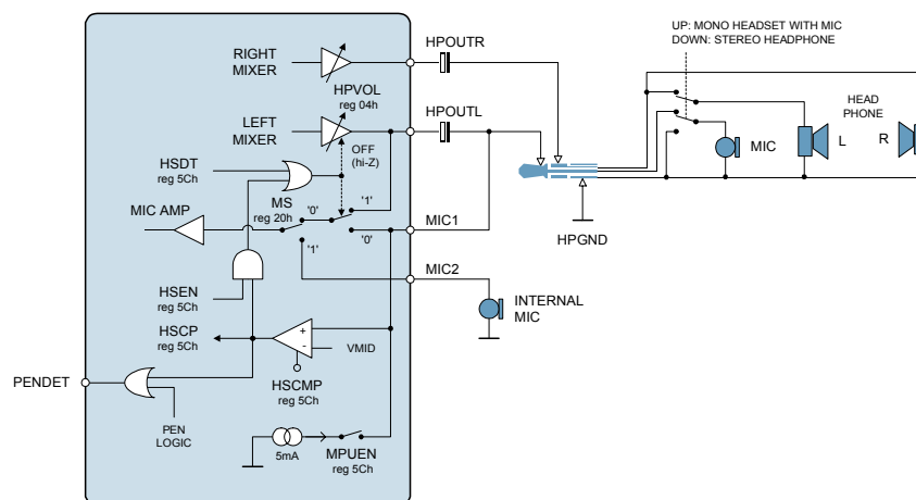
Figure 10 Headset Autodetect
