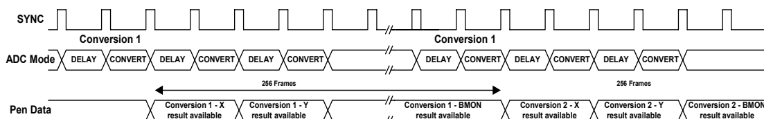
Figure 23 Control of ADC Conversions : Continuous Method
