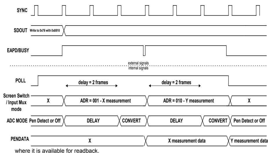
Figure 21 Control of ADC conversions : Polling Method
