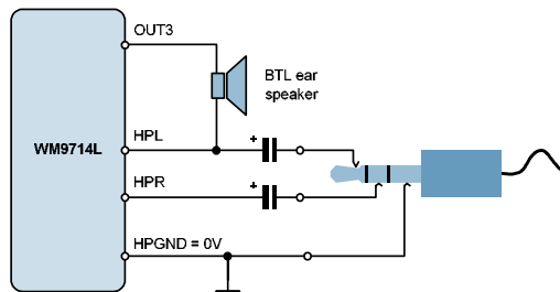
Figure 30 Combined Headset / BTL Ear Speaker
