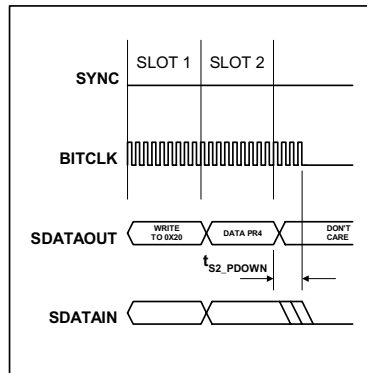
Figure 23 AC-Link Powerdown Timing
