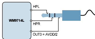
Figure 28 Capless Headphone Output Circuit Diagram
