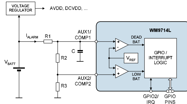
Figure 17 Battery Alarm Example Schematic
