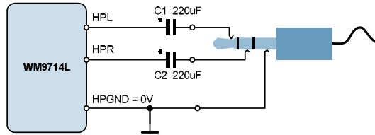
Figure 27 Simple Headphone Output Circuit Diagram
