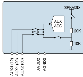
Figure 16 AUX ADC Switch Matrix
