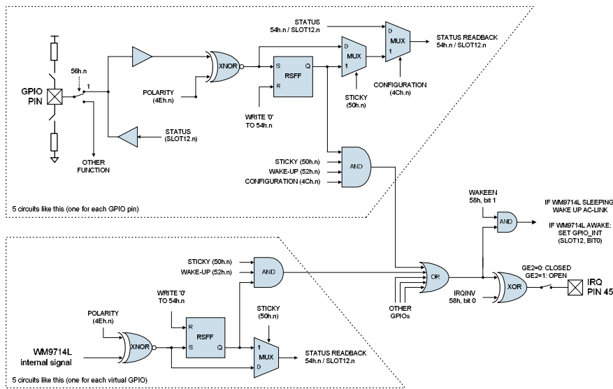
Figure 19 GPIO Logic
