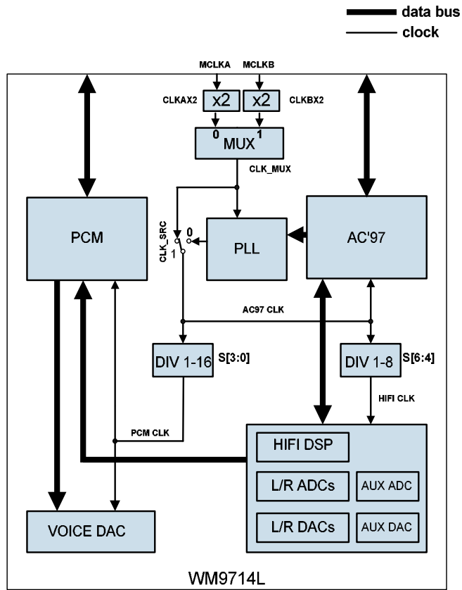
Figure 2 Clocking Architecture for WM9714L
