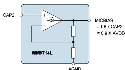
Figure 14 Microphone Bias Schematic
