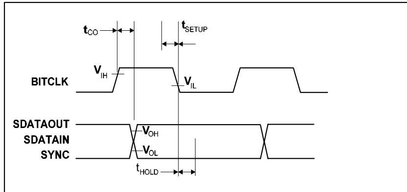
Figure 21 Data Setup and Hold (50pF External Load)
