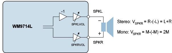
Figure 29 Speaker Output Connection (INV = 1)
