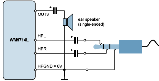
Figure 31 Combined Headset / Single-ended Ear Speaker
