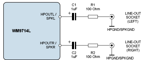
Figure 26 Recommended Circuit for Line Output
