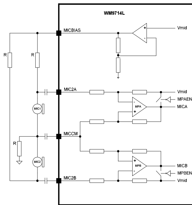
Figure 13 Dual Microphone Configuration
