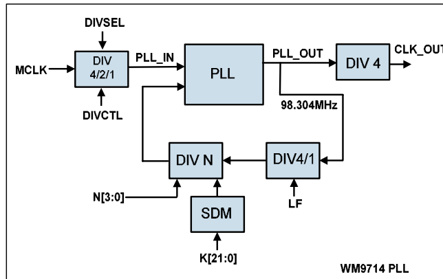
Figure 3 PLL Architecture
