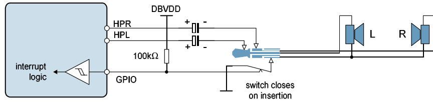
Figure 32 Jack Insert Detection Circuit
