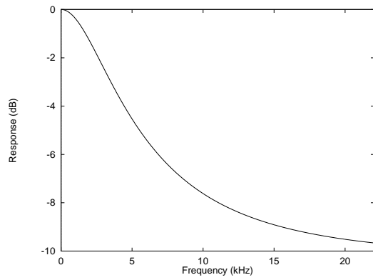
Figure 29 De-Emphasis Frequency Response (44.1kHz)
