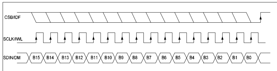
Figure 20 3-Wire SPI Compatible Interface
