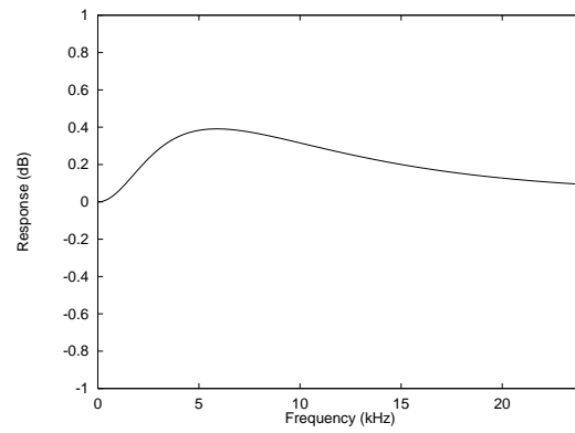
Figure 32 De-Emphasis Error (48kHz)
