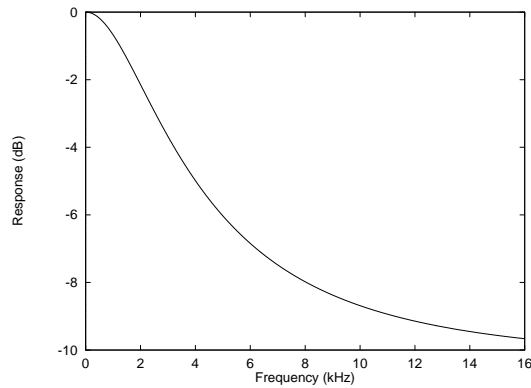
Figure 27 De-Emphasis Frequency Response (32kHz)
