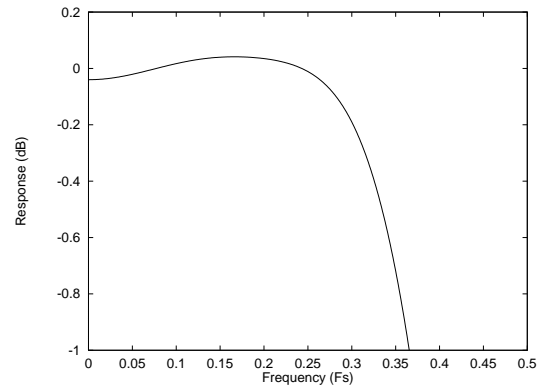
Figure 24 DAC Digital Filter Ripple – 192kHz
