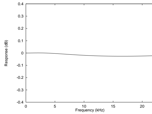
Figure 30 De-Emphasis Error (44.1kHz)
