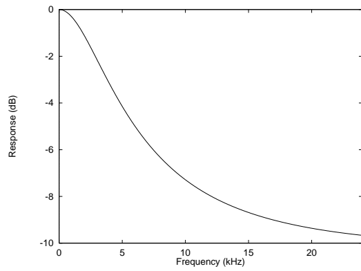
Figure 31 De-Emphasis Frequency Response (48kHz)
