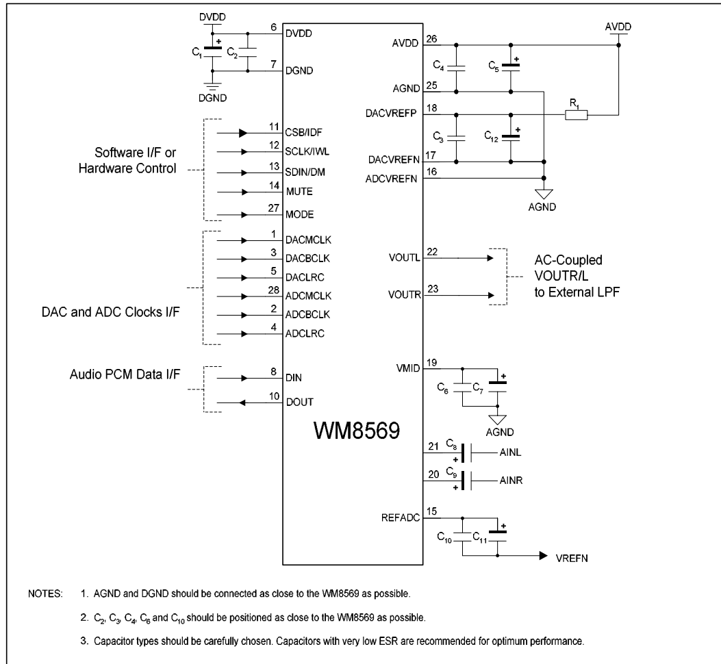
Figure 33 Recommended External Components Diagram
