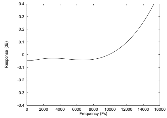
Figure 55 De-emphasis Error (32kHz)
