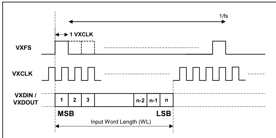
Figure 26 Voice Interface Mono Mode (mode B, PLRP=0)
