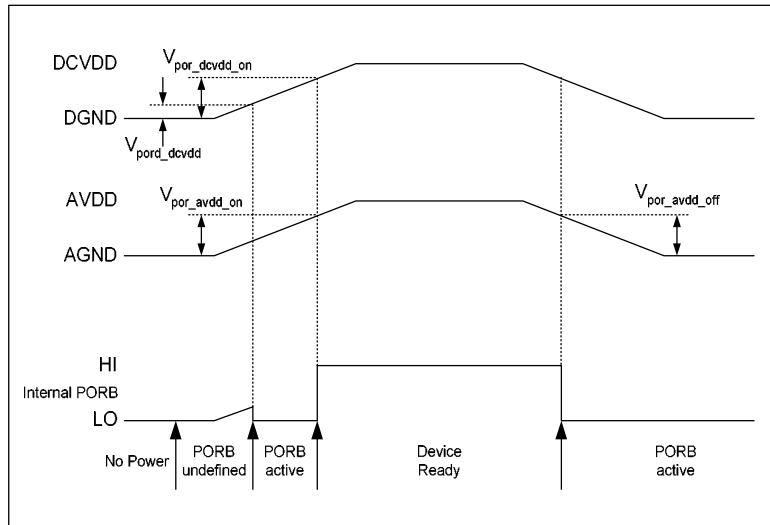
Figure 7 Typical Power-Up Sequence
