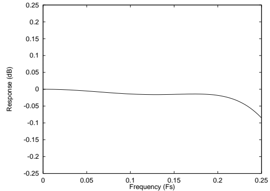
Figure 41 ADC Digital Filter Ripple – Type 2
