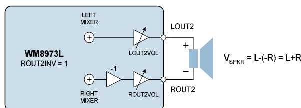
Figure 14 Speaker Output Connection
