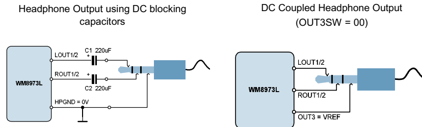
Figure 13 Recommended Headphone Output Configurations
