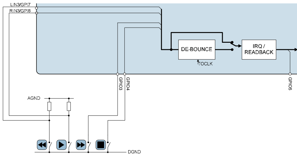
Figure 21 Example of Button Control Using GPIO Pins
