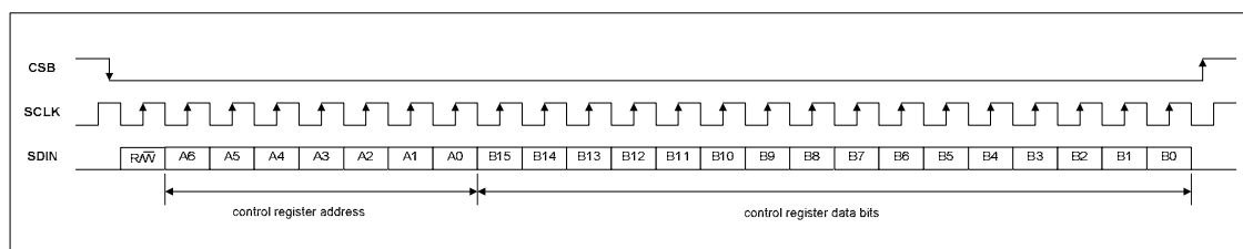
Figure 55 3-Wire Serial Control Interface
