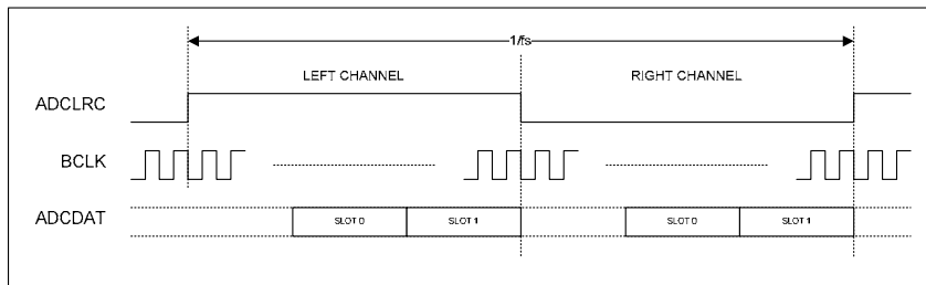
Figure 42 TDM in Right-Justified Mode
