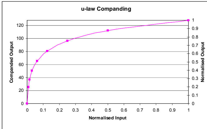
Figure 48 \mu -Law Comanding
