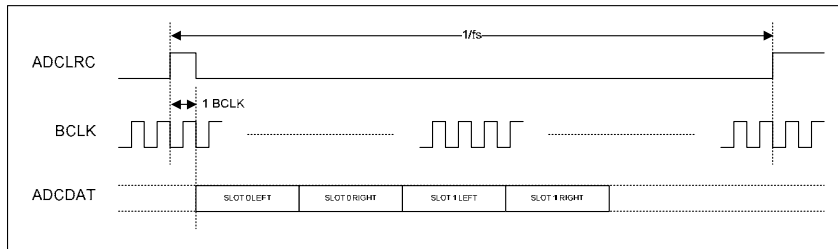
Figure 45 TDM in DSP Mode A
