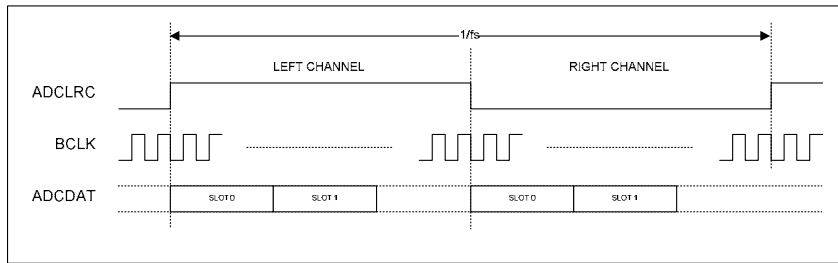
Figure 43 TDM in Left-Justified Mode
