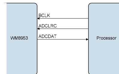
Figure 30 Slave Mode
