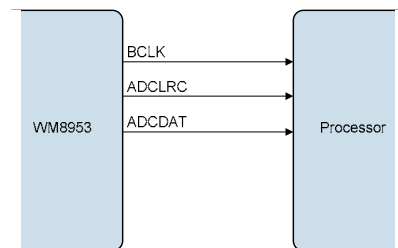
Figure 29 Master Mode
