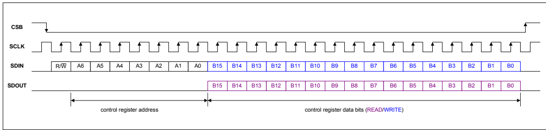
Figure 56 4-Wire Readback (Push 0/1)
