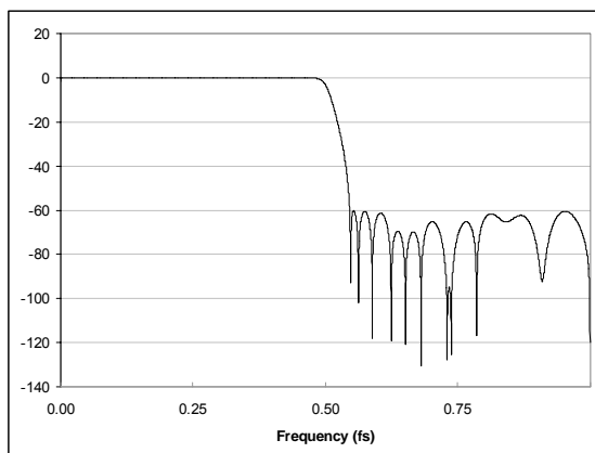
Figure 59 ADC Digital Filter Frequency Response
