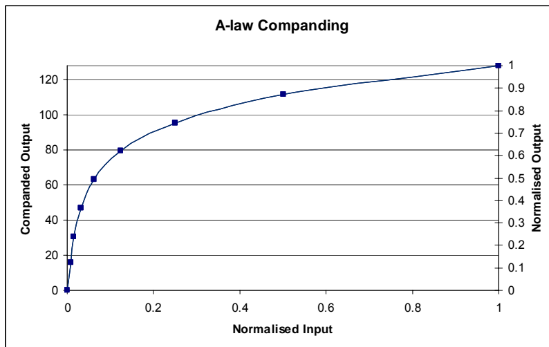
Figure 49 A-Law Comanding
