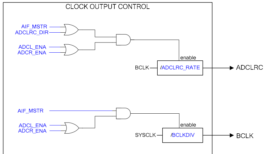
Figure 47 Clock Output Control
