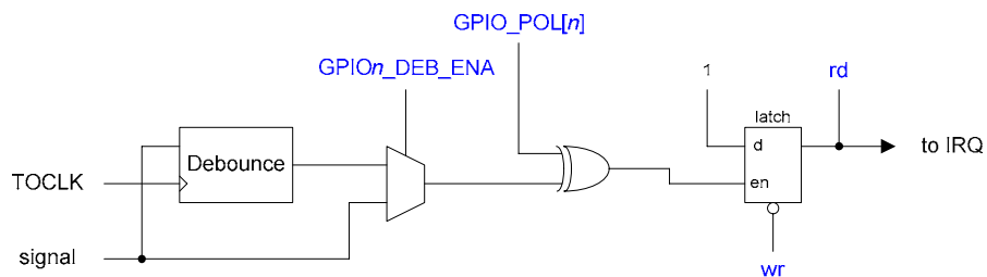
Figure 24 GPIO Function
