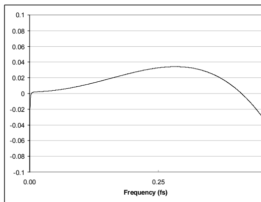
Figure 60 ADC Digital Filter Ripple
