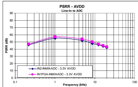
AVDD – Line-In to ADC
