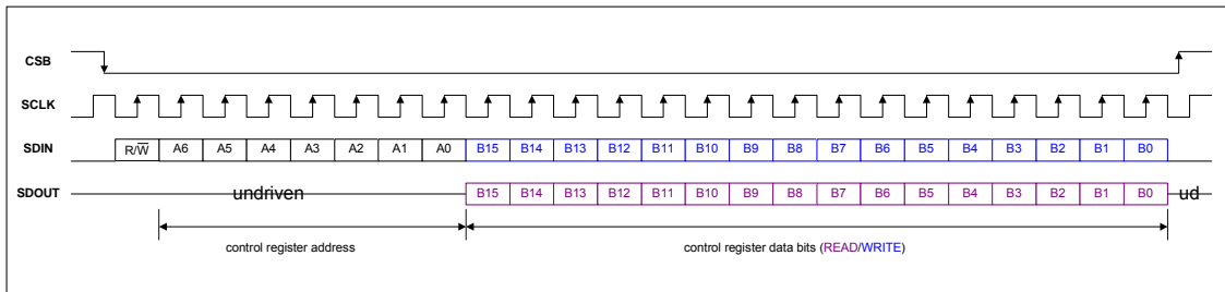
Figure 57 4-Wire Readback (wired-OR)
