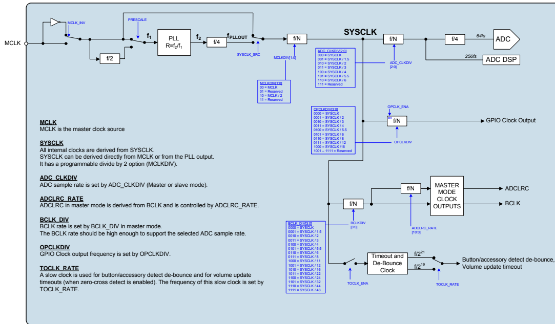
Figure 50 Clocking Scheme
