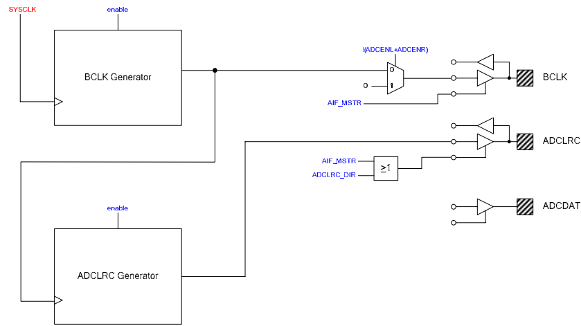
Figure 31 Audio Interface Output Control
