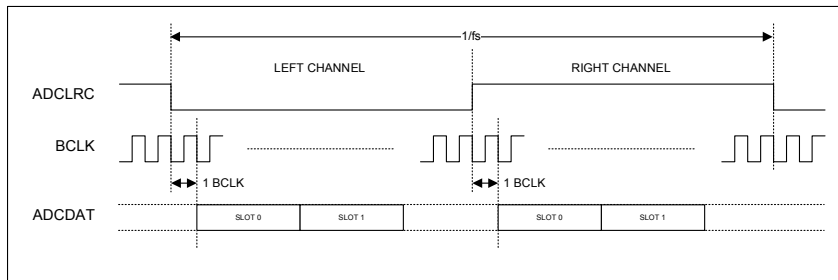
Figure 44 TDM in I 2 S Mode
