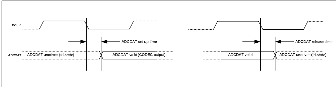
Figure 5 Digital Audio Data Timing - TDM Mode
