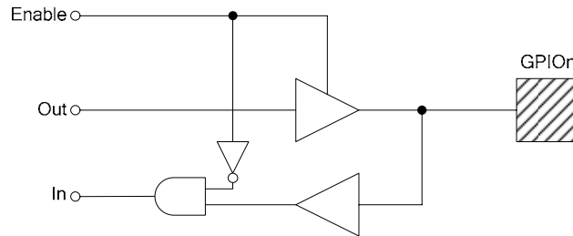
Figure 23 GPIO Pad
