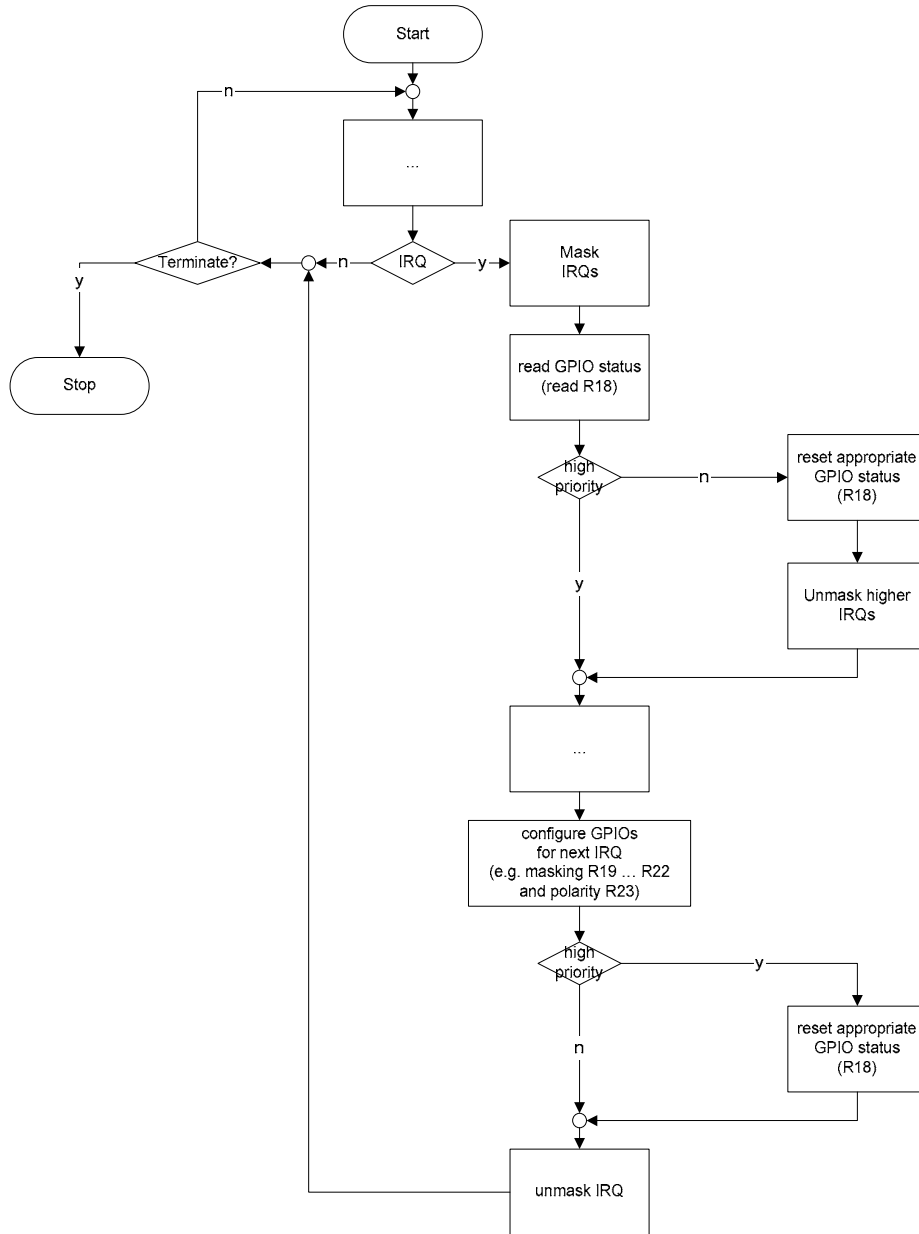
Figure 28 GPIO IRQ Handling
