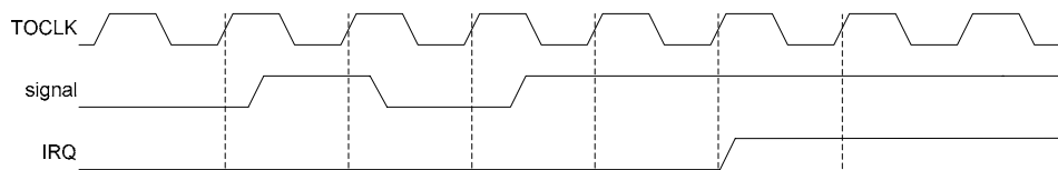
Figure 26 GPIO De-bounce
