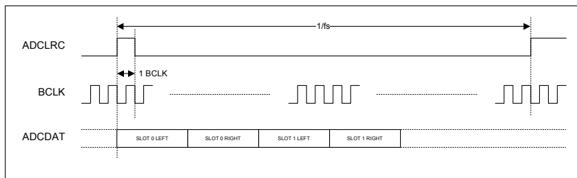
Figure 46 TDM in DSP Mode B
