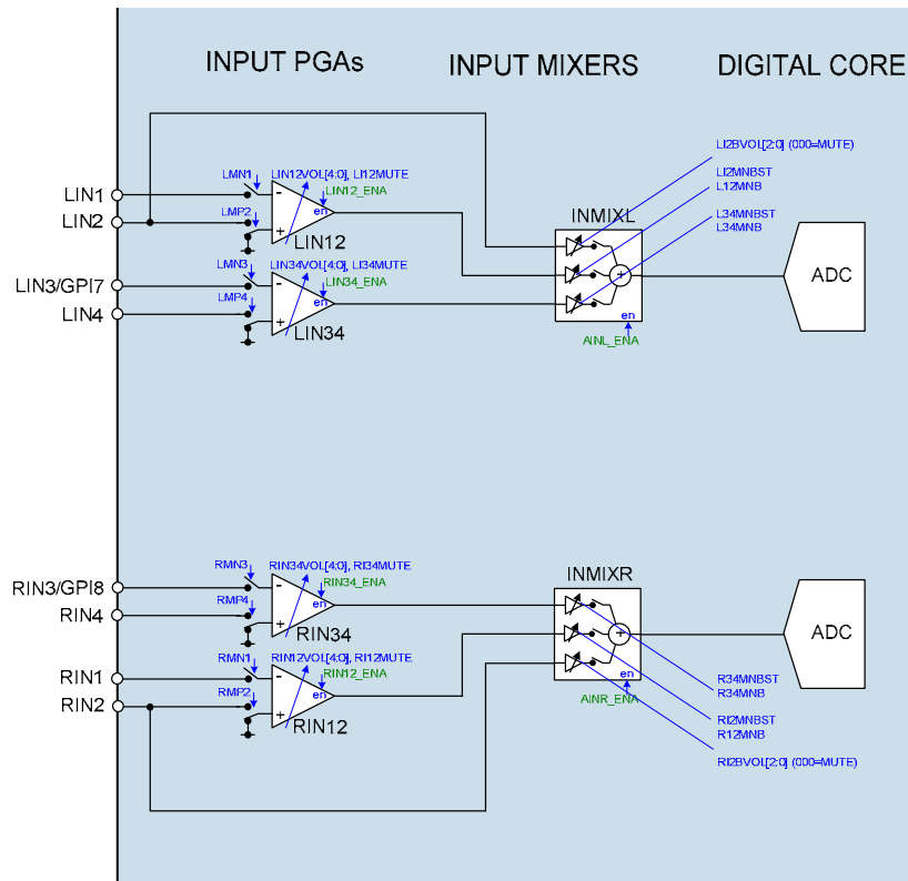
Figure 14 Control Registers for Input Signal Path
