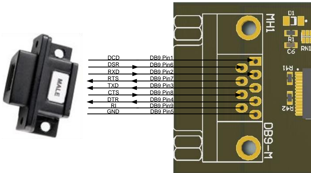
Figure 2.2 – DB9-USB-RS232-M Connection illustration
