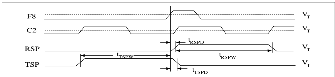
Figure 19. Output Timing
