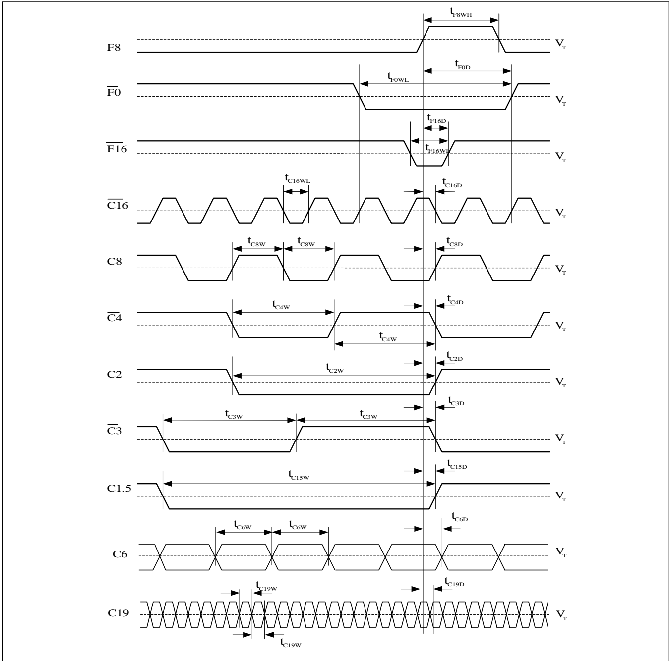
Figure 19. Output Timing
