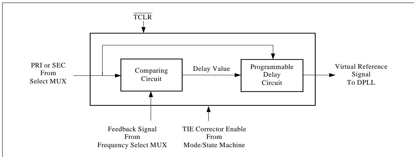
Figure 3. TIE Corrector
