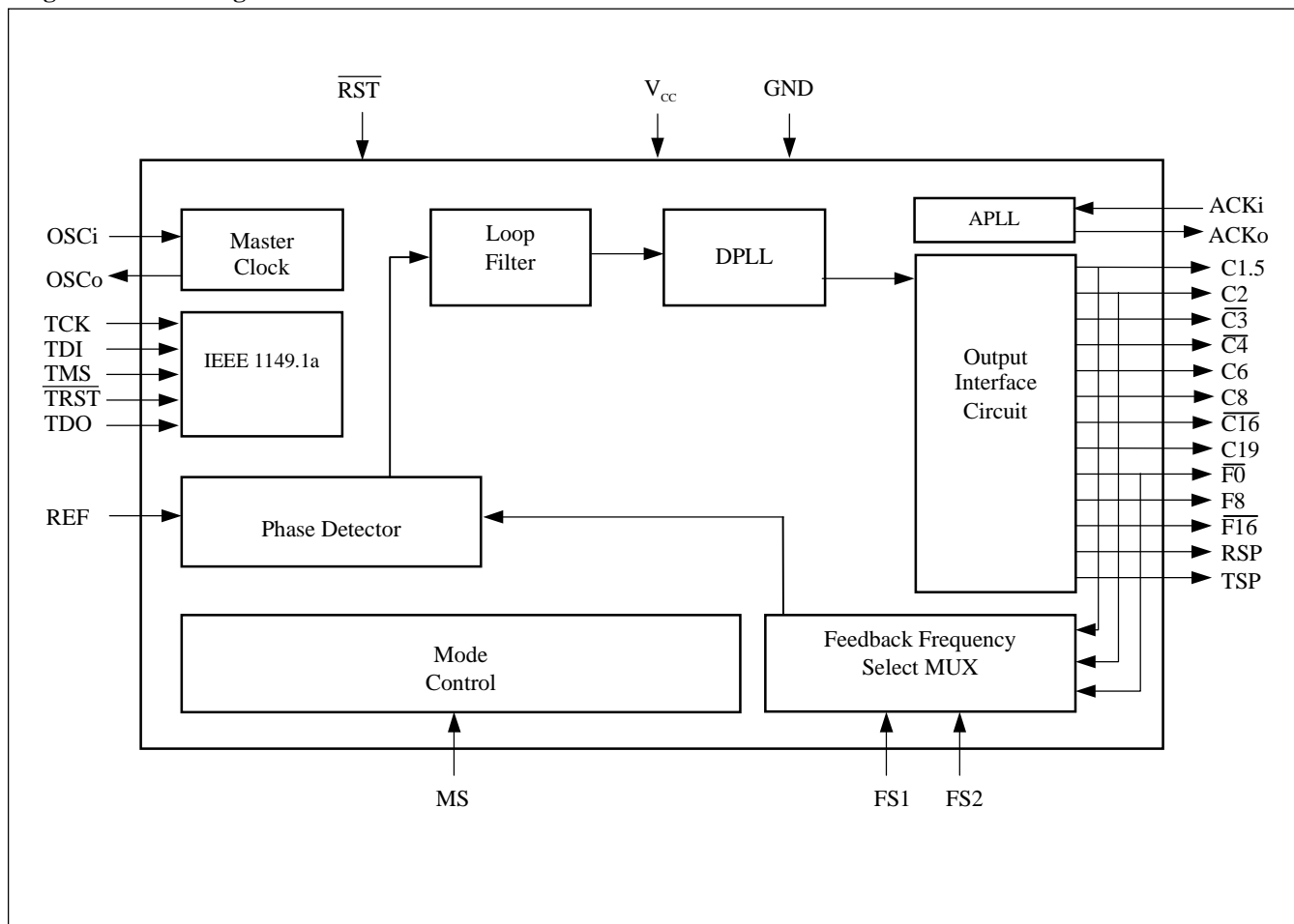
Figure 1. Block Diagram
