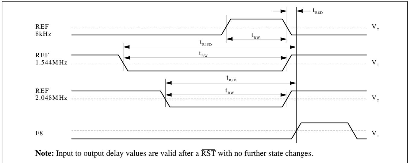
Figure 9. Timing Information for PT7A4401B
