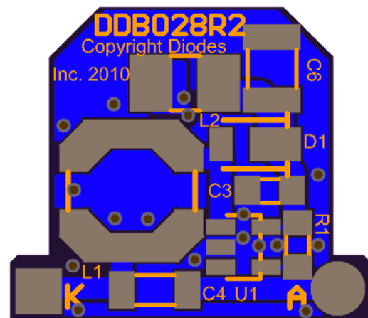
Figure 38. Bottom Layer
