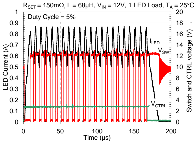
Figure 11. PWM dimming
