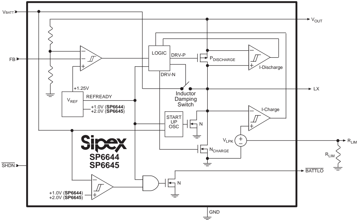
Figure 27. Internal Block Diagram of the SP6644/6645
