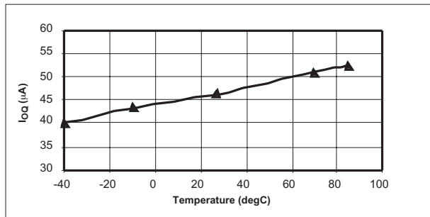
Figure 15. I_{oq} Pin Quiescent Current vs. Temperature, ( V_{out}=3.3\text{V} )
