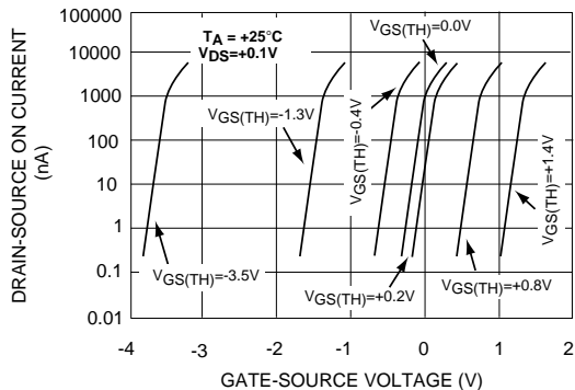
SUBTHRESHOLD FORWARD TRANSFER CHARACTERISTICS
