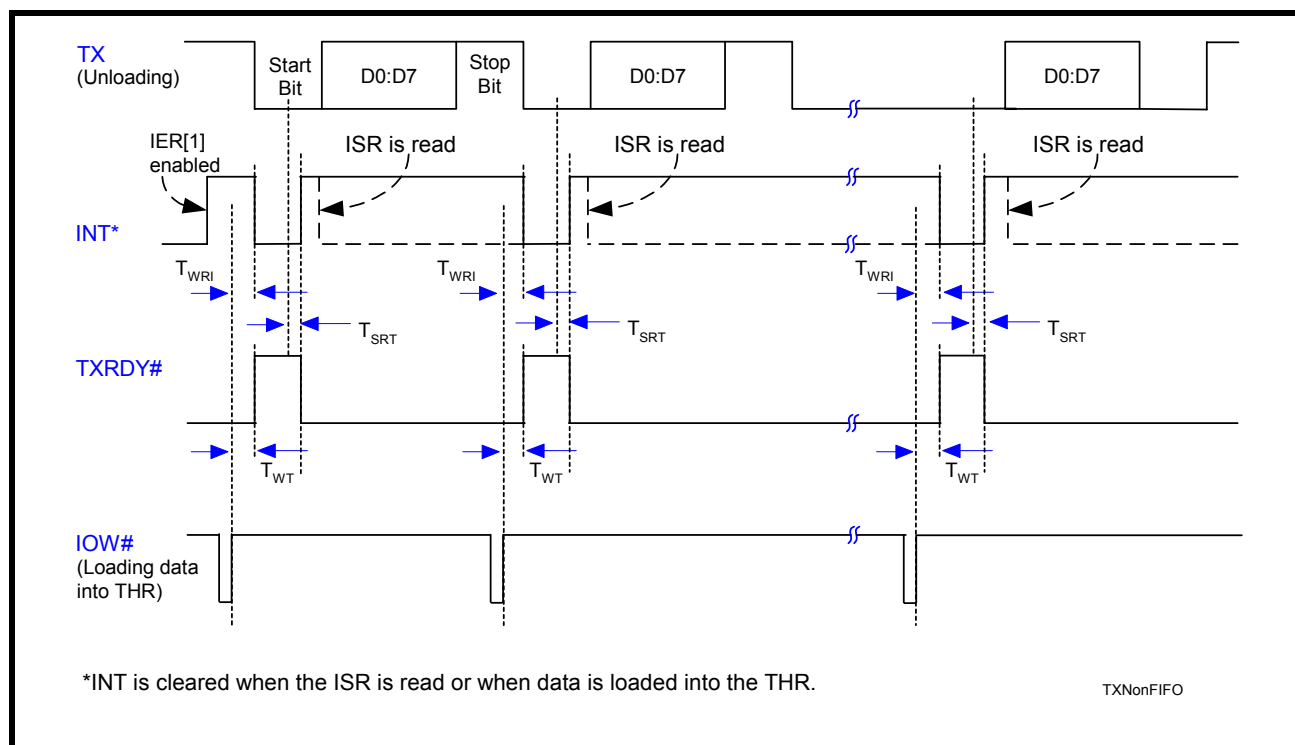
FIGURE 27. TRANSMIT READY &amp; INTERRUPT TIMING [Non-FIFO Mode]
