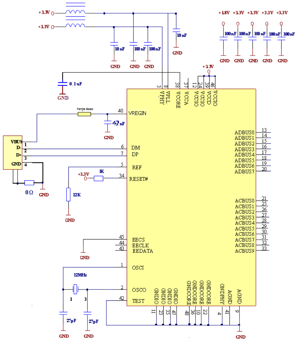
Figure 6.1 Bus Powered Configuration Example 1
