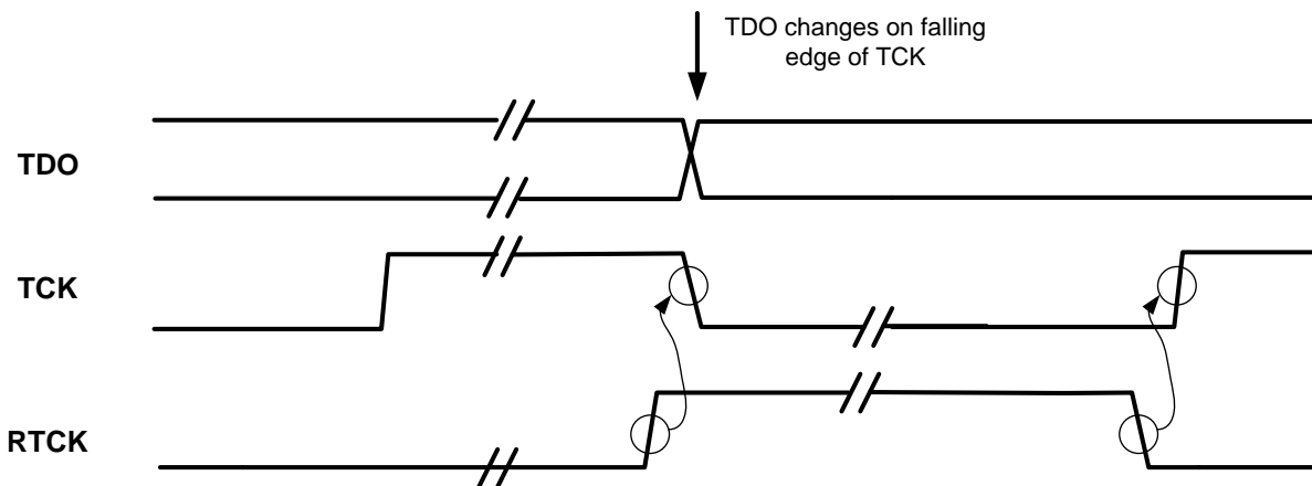
Figure 4.16: Adaptive Clocking waveform.
