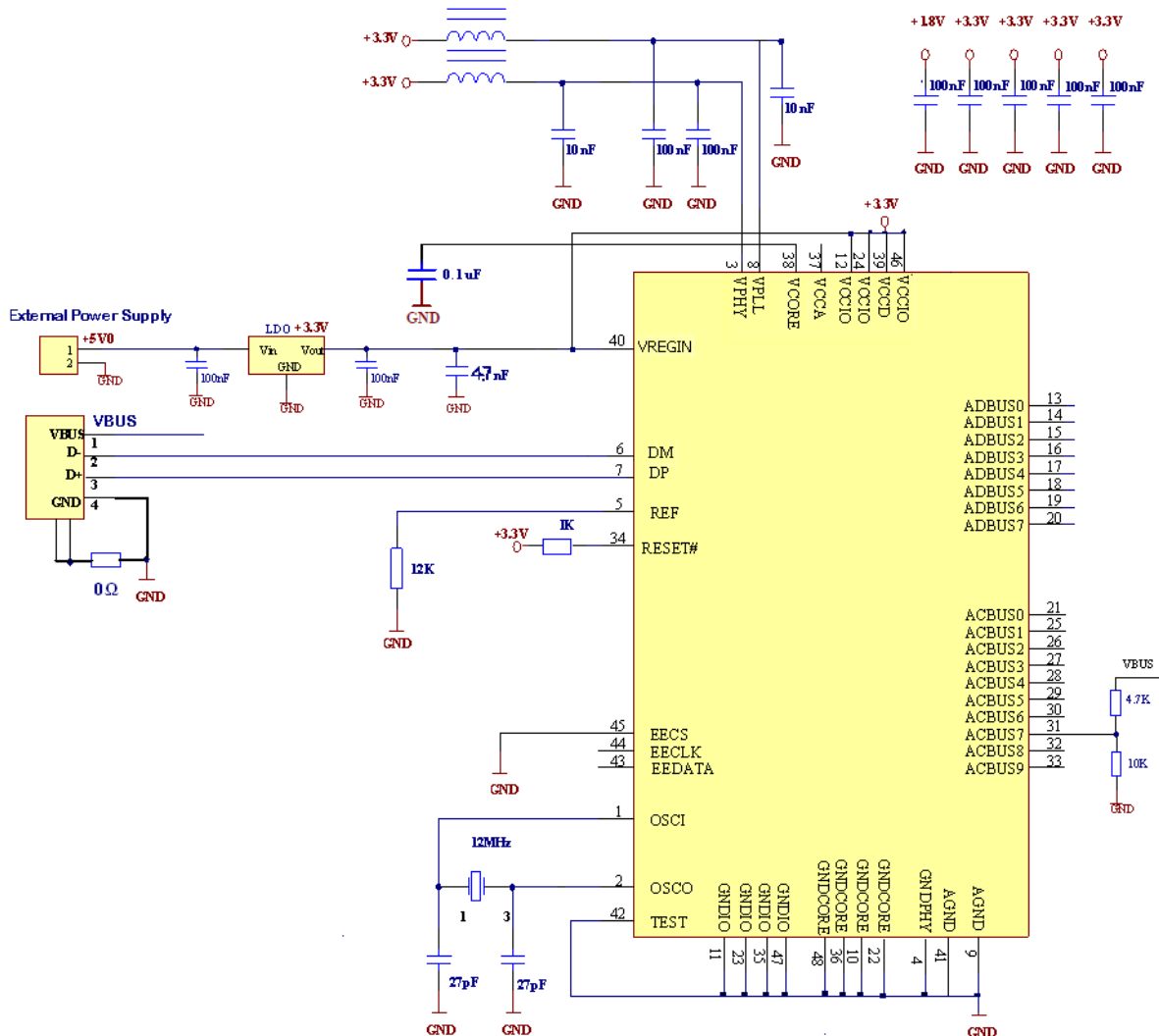
Figure 6.3 Self Powered Configuration Example 2
