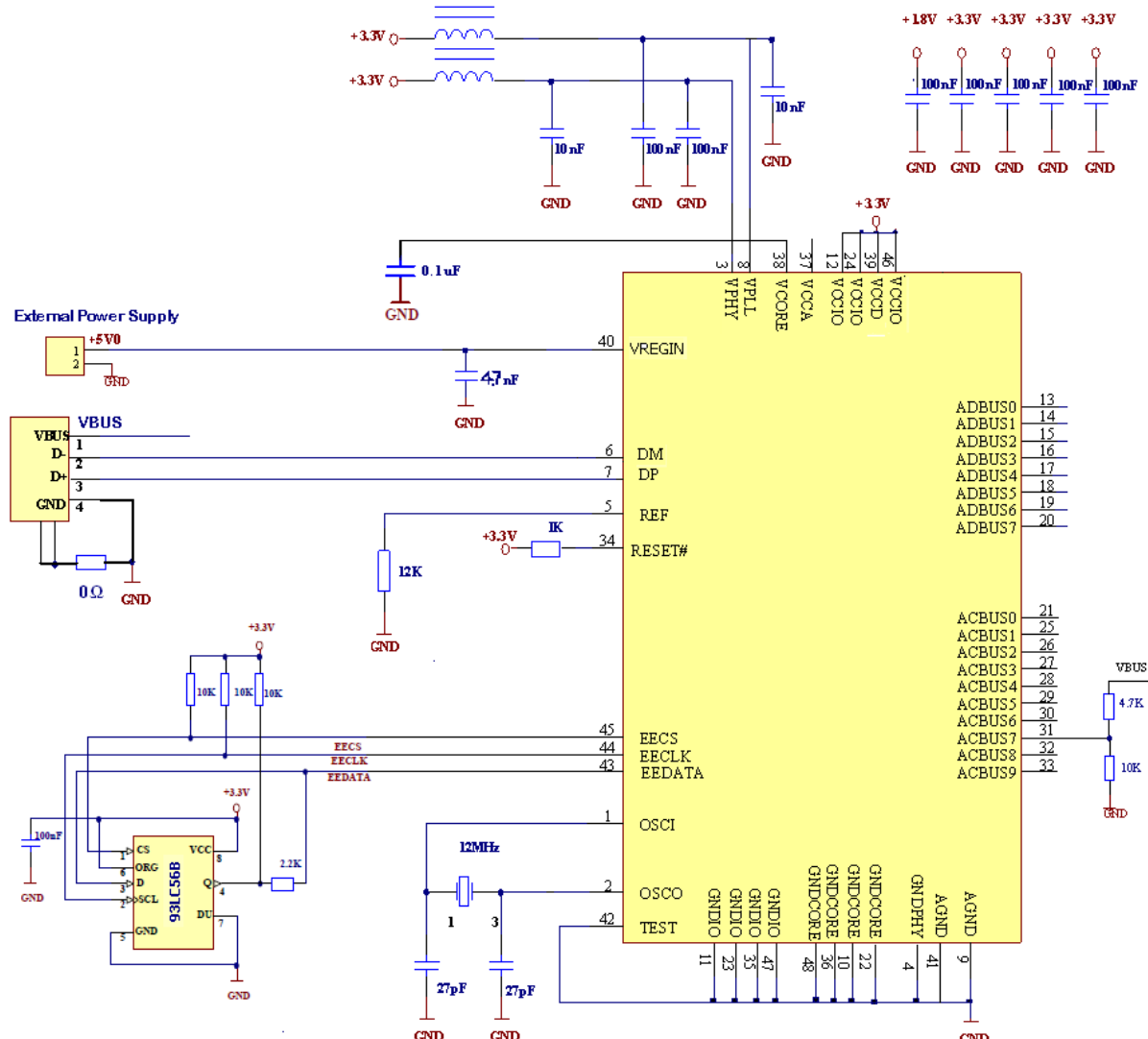
Figure 7.1 EEPROM Interface
