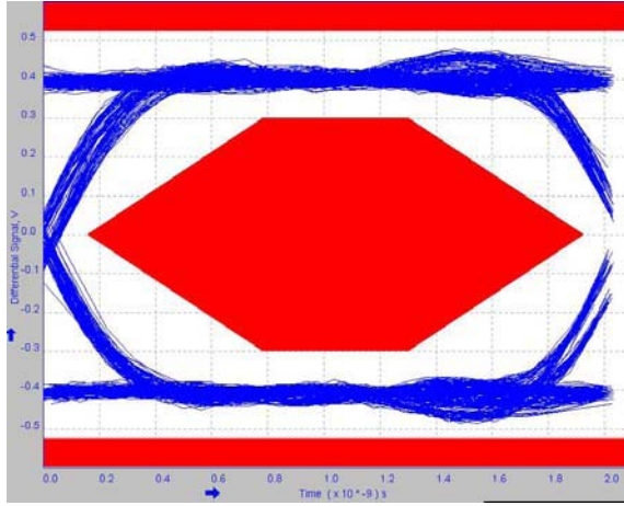
Figure 3. Reference Near End Eye Diagram (Path Through Dedicated Line, Temp = 25°C)
