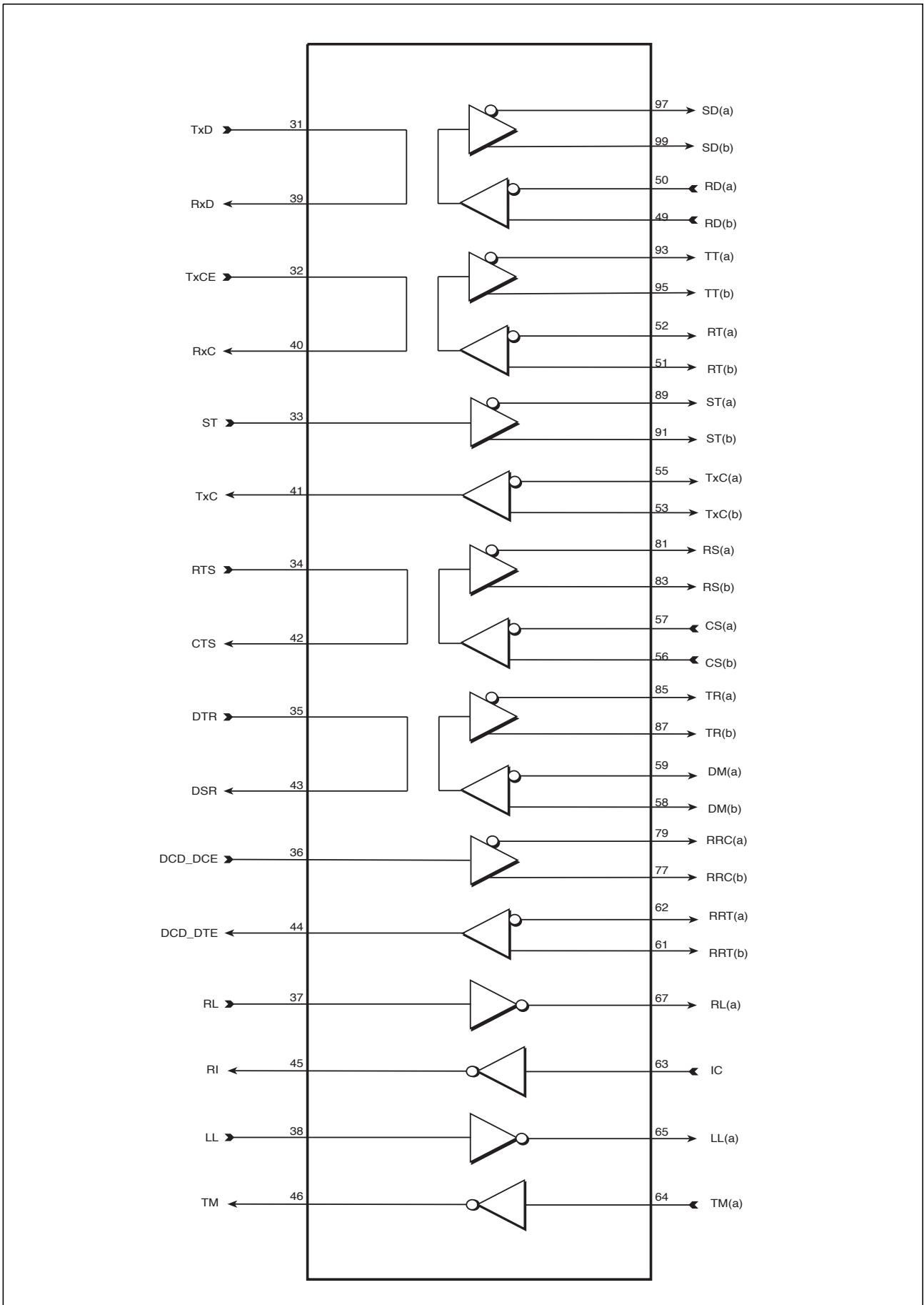
Figure 50. Loopback Path
