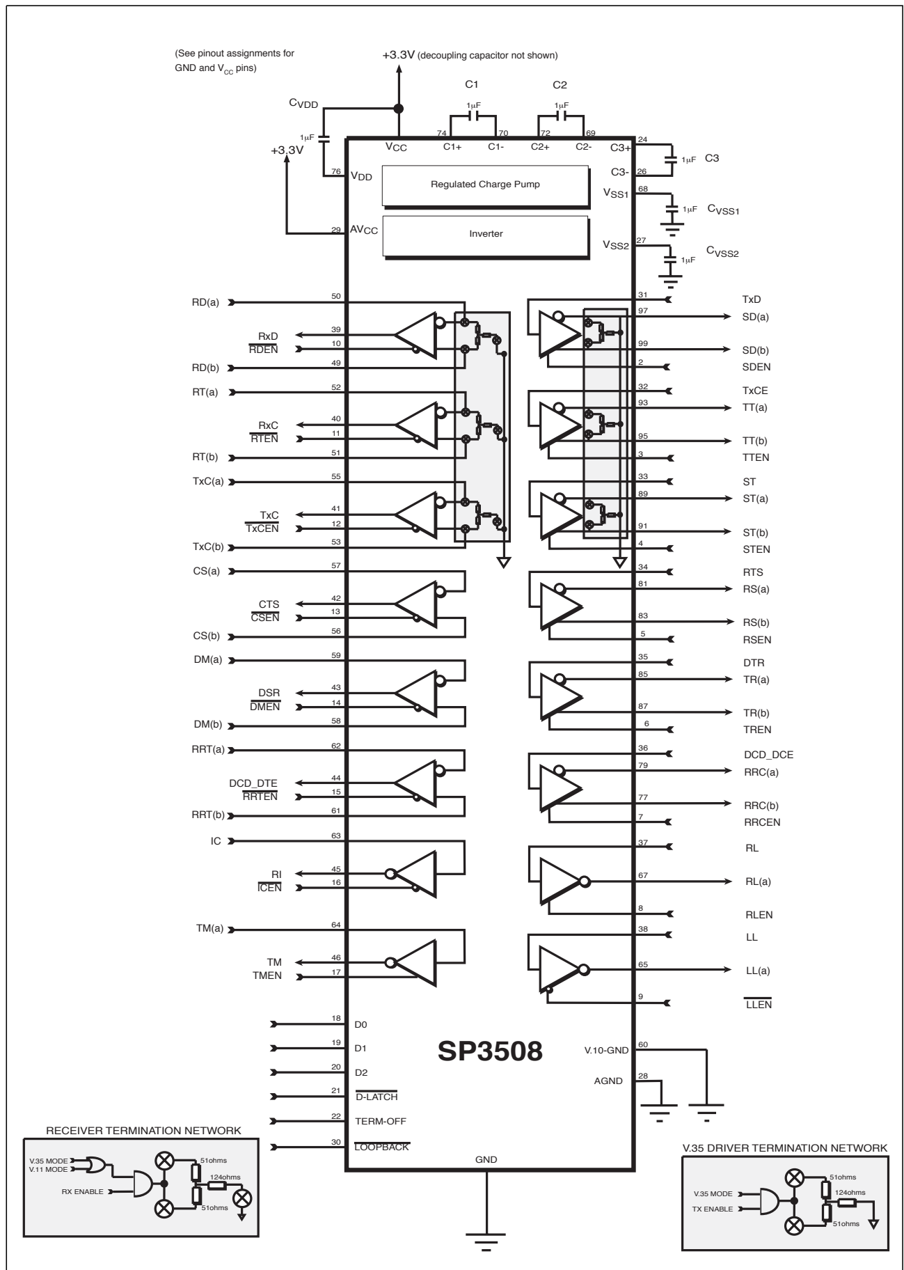
Figure 44. Functional Diagram
