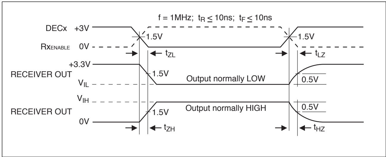
Figure 38. Receiver Enable and Disable Times
