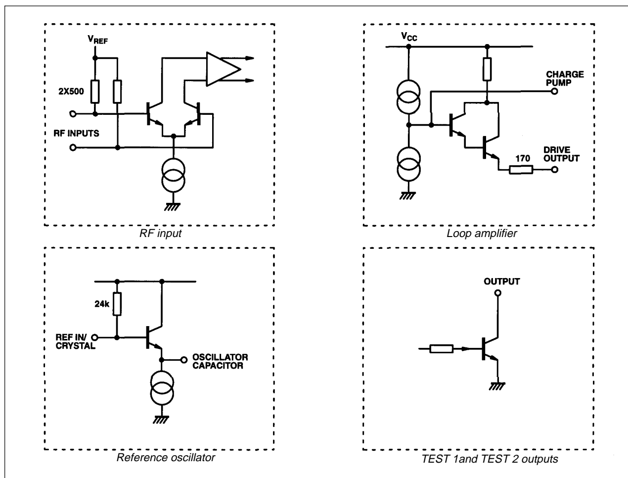
Fig.7 SP5070 input/output interface circuits
