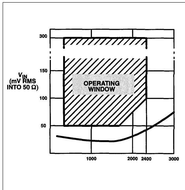
Fig.5 Typical input sensitivity
