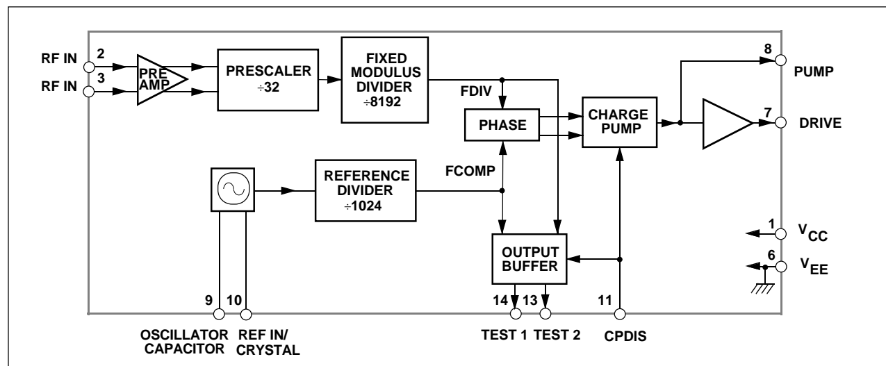
Fig.2 Block diagram of SP5070
