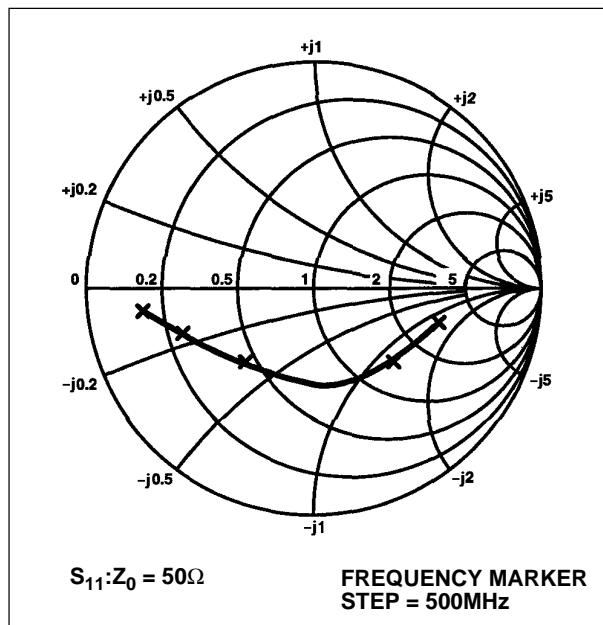
Fig.6 Typical input impedance
