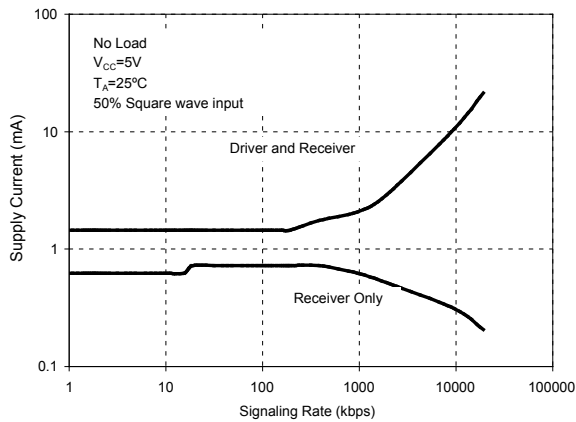
Supply Current vs Signaling Rate (SP3086-SP3088)
