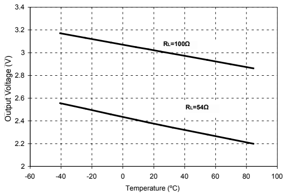
Driver Differential Output Voltage vs Temperature
