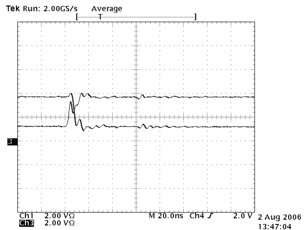
Driver Output Waveform Low to High (SP3086-SP3088)
