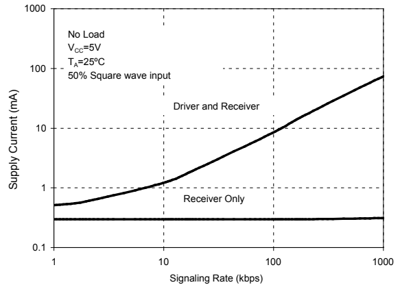
Supply Current vs Signaling Rate (SP3083-SP3085)
