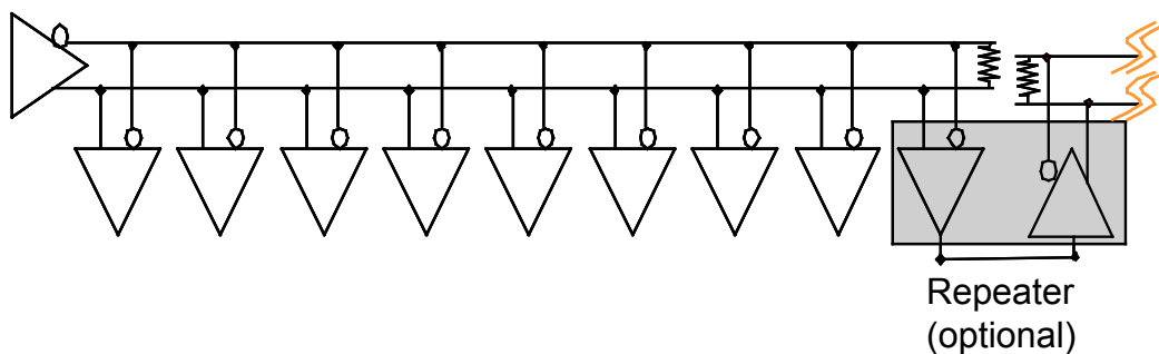
Point to Multi-Point Repeater
