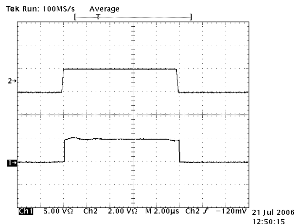
Receiver Propagation Delay (SP3080-SP3082)
