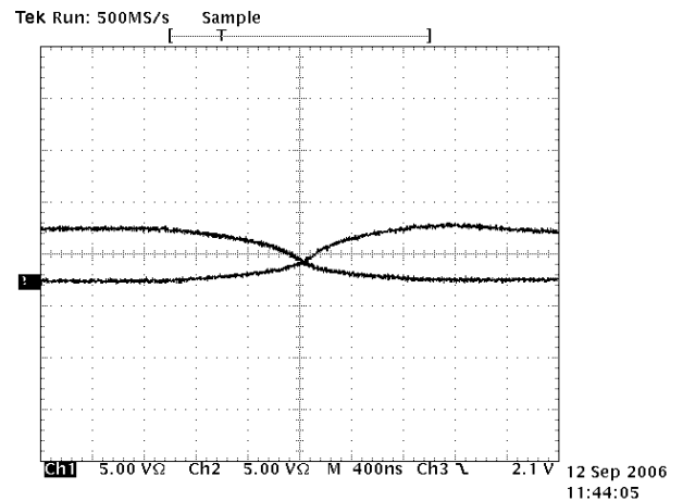
Driver output Waveform High to Low (SP3080-SP3082)
