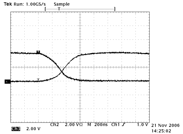
Driver Output Waveform High to Low (SP3083-SP3085)
