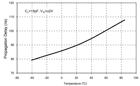
Receiver Average Propagation Delay vs Temperature (SP3080-SP3082)
