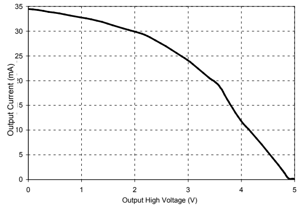
Output Current vs Receiver Output High Voltage
