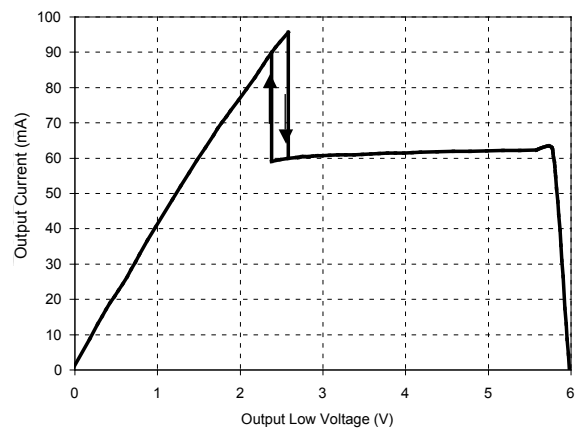
Output Current vs Driver Output Low Voltage
