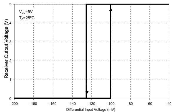
Receiver Output Voltage vs Differential Input Voltage
