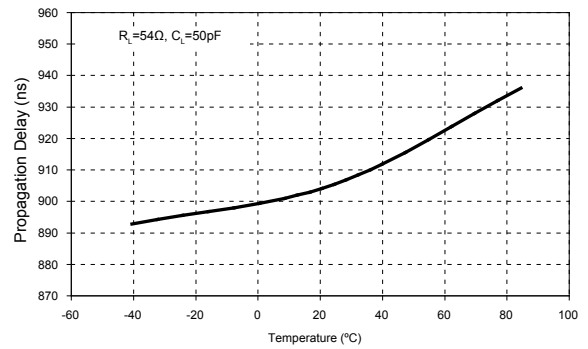
Driver Average Propagation Delay vs Temperature (SP3080-SP3082)
