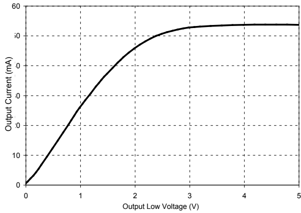
Output Current vs Receiver Low Voltage
