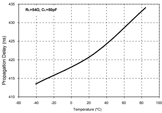
Driver Average Propagation Delay vs Temperature (SP3083-SP3085)
