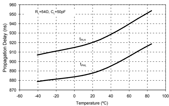
Driver Propagation Delay vs Temperature (SP3080-SP3082)
