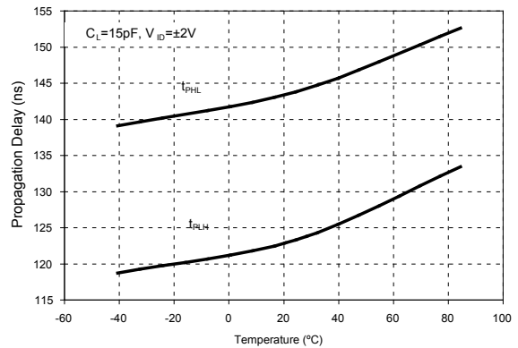
Receiver Propagation Delay vs Temperature (SP3083-SP3085)
