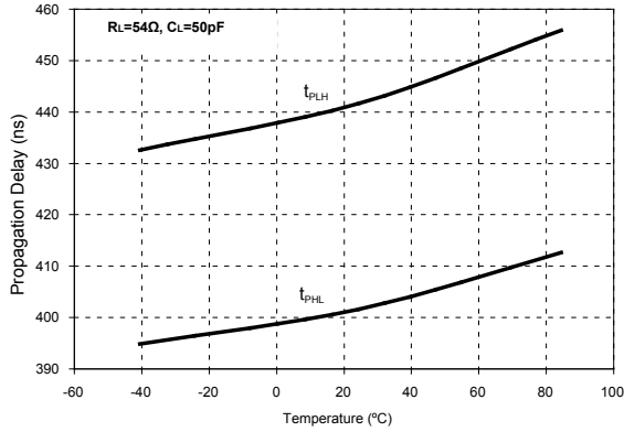
Driver Propagation Delay vs Temperature (SP3083-SP3085)
