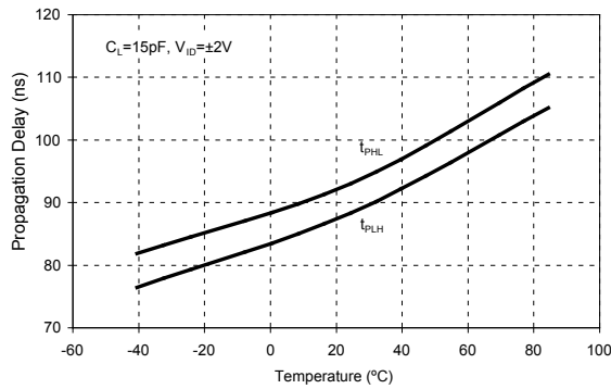
Receiver Propagation Delay vs Temperature (SP3080-SP3082)
