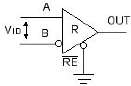
Receiver DC Test Circuit
