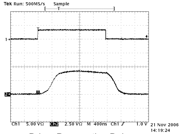
Driver Propagation Delay (SP3083-SP3085)
