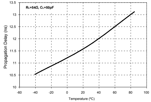
Driver Average Propagation Delay vs Temperature (SP3086-SP3088)
