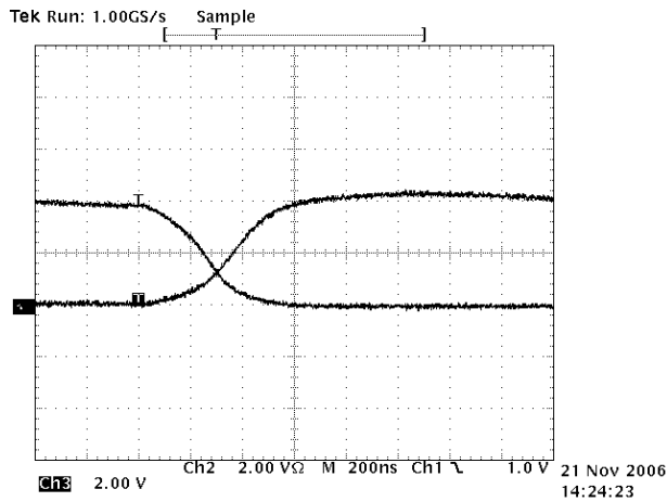
Driver Output Waveform Low to High (SP3083-SP3085)
