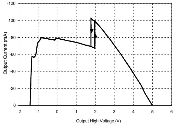
Output Current vs Driver Output High Voltage
