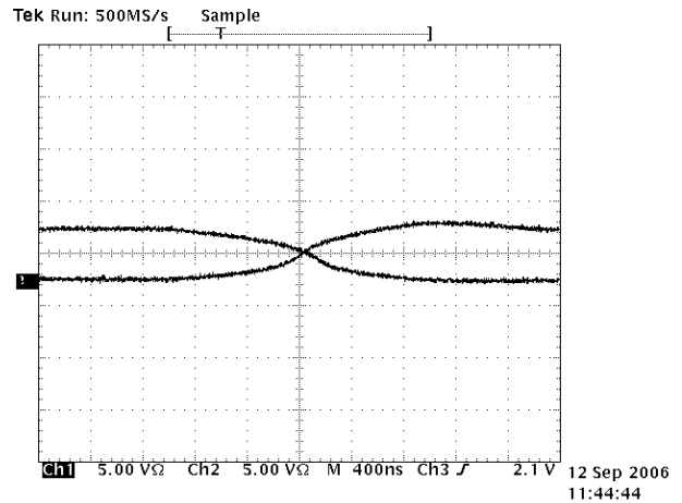
Driver output Waveform Low to High (SP3080-SP3082)
