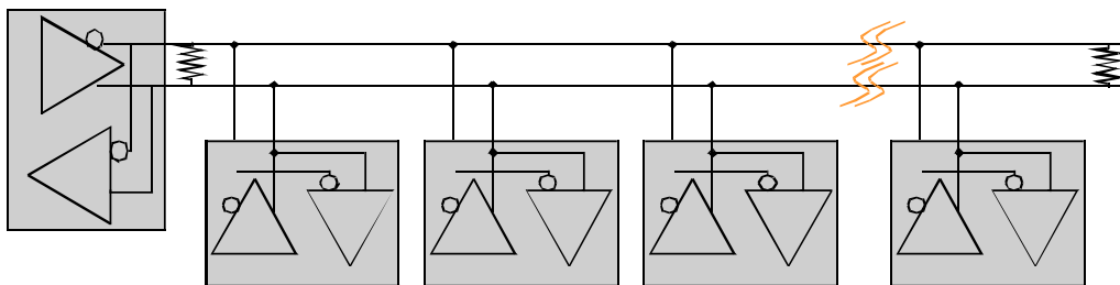
Half-Duplex Network
