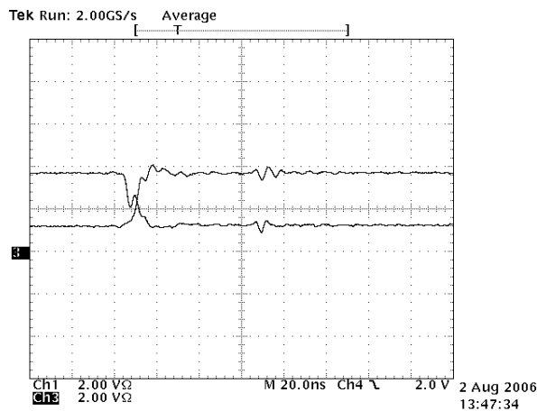
Driver Output Waveforms High to Low (SP3086-SP3088)
