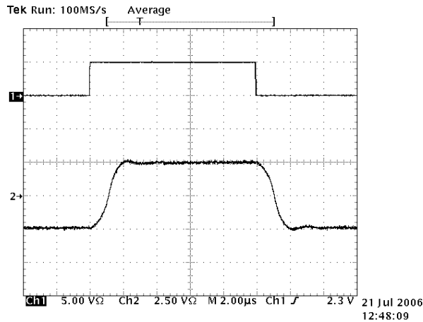
Driver Propagation Delay (SP3080-SP3082)
