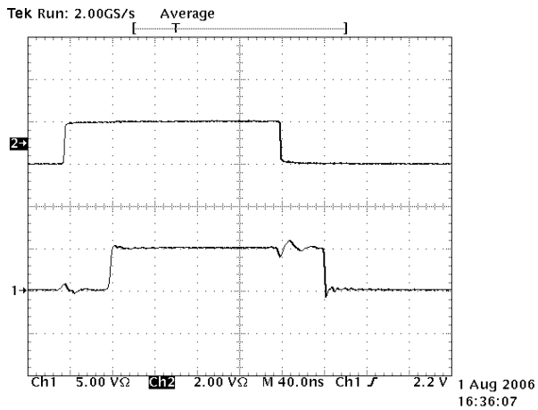
Receiver Propagation Delay (SP3086-SP3088)
