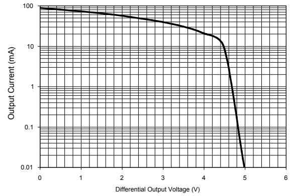
Driver Output Current vs Differential Output Voltage
