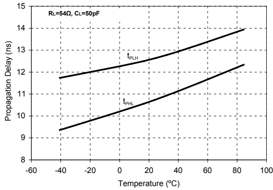
Driver Propagation Delay vs Temperature (SP3086-SP3088)
