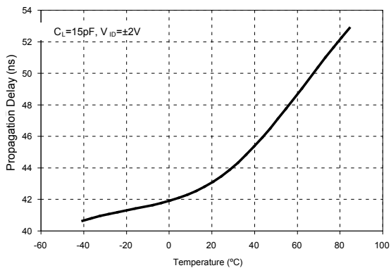
Receiver Average Propagation Delay vs Temperature (SP3086-SP3088)
