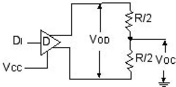
Driver DC Test Circuit
