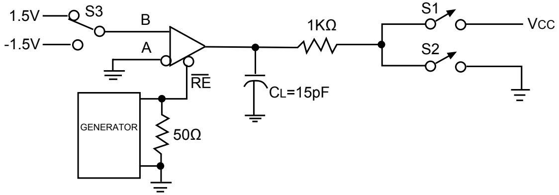
Receiver Enable and Disable Times Test Circuit
