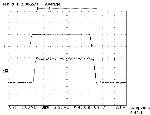
Driver Propagation Delay (SP3086-SP3088)
