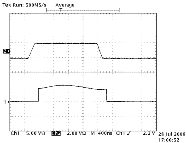
Receiver Propagation Delay (SP3083-SP3085)
