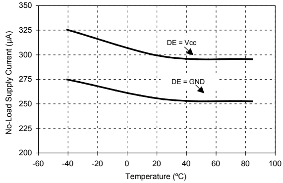
No-load Supply Current vs Temperature
