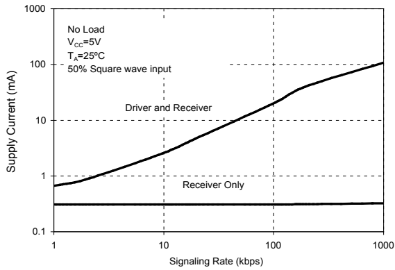
Supply Current vs Signaling Rate (SP3080-SP3082)
