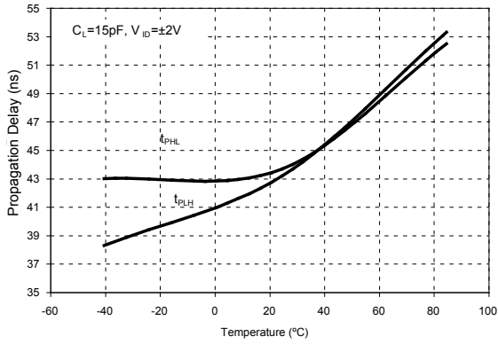
Receiver Propagation Delay vs Temperature (SP3086-SP3088)
