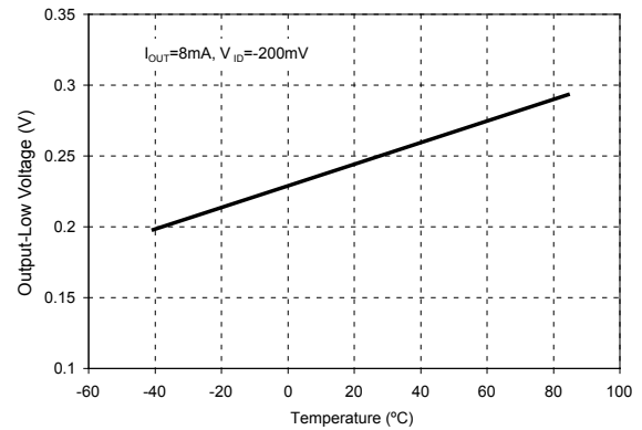
Receiver Output Low Voltage vs Temperature
