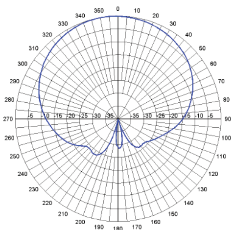
SP2327-15XP90NUF azimuth plane
