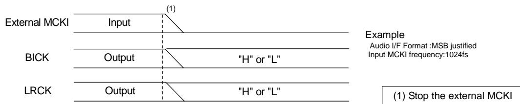
Figure 82. Clock Stopping Sequence (5)
