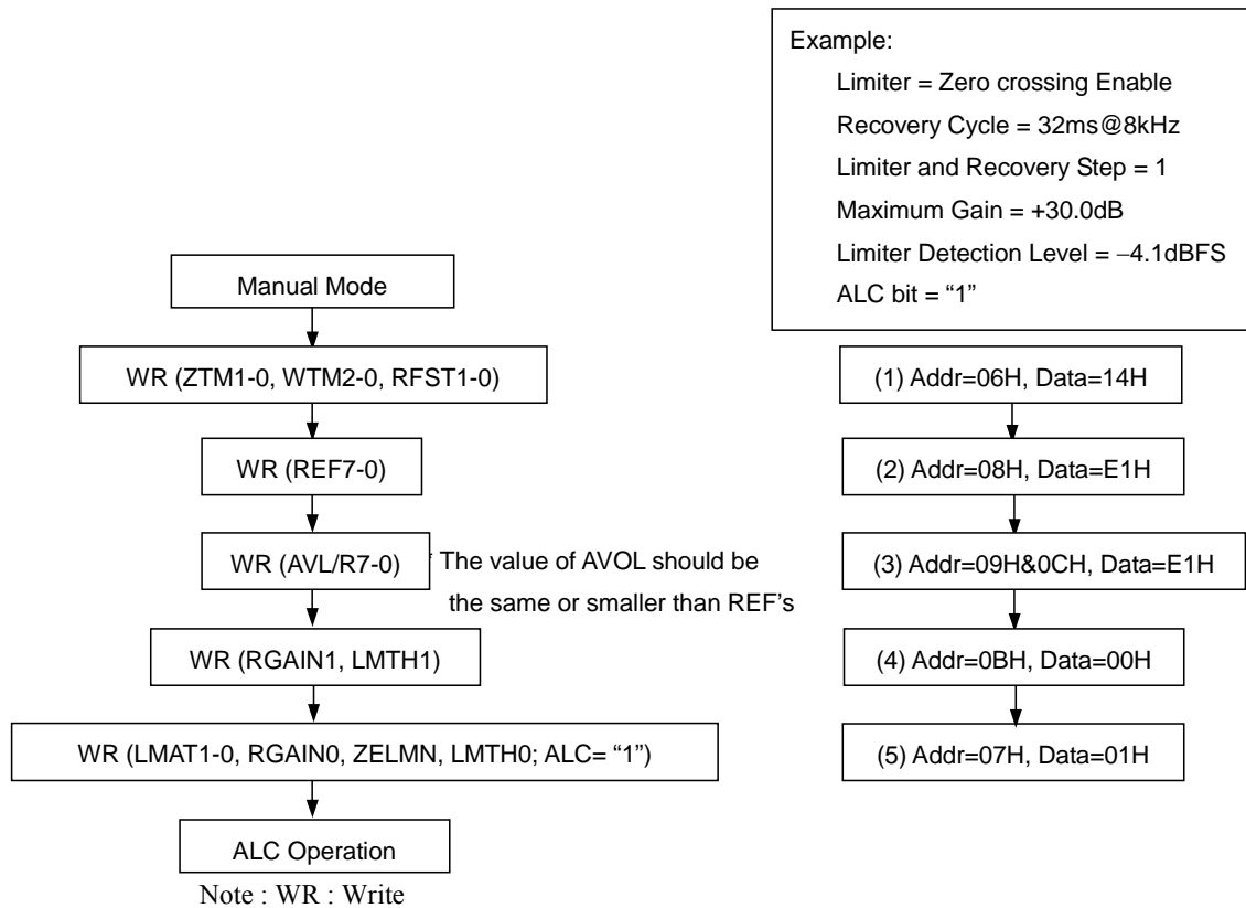
Figure 47. Registers set-up sequence at ALC operation
