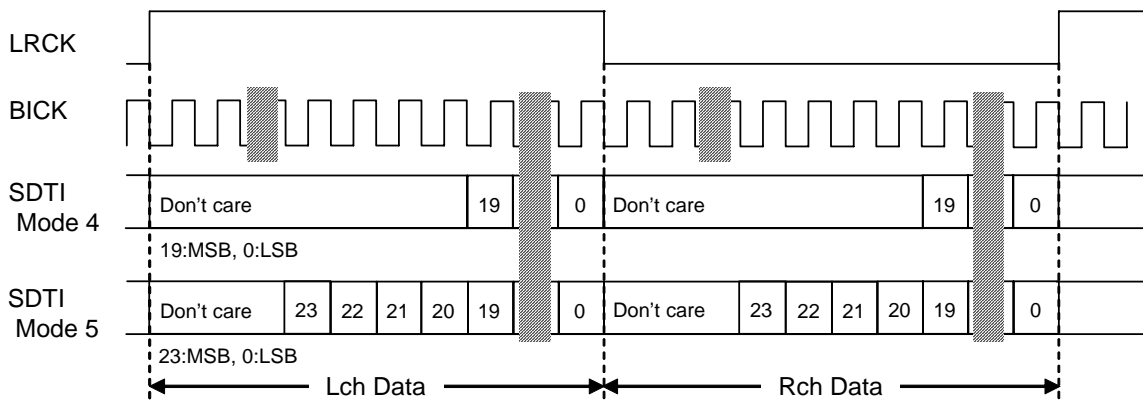
Figure 35. Mode 4, 5 Timing
