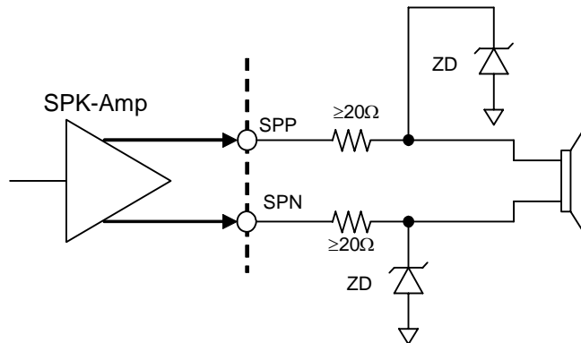
Figure 56. Speaker Output Circuit (Load Capacitance &gt; 30pF)
