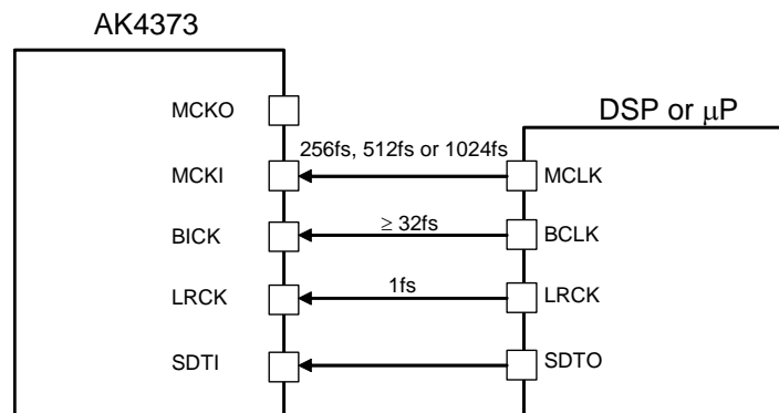
Figure 28. EXT Slave Mode
