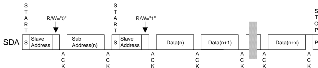
Figure 64. RANDOM ADDRESS READ
