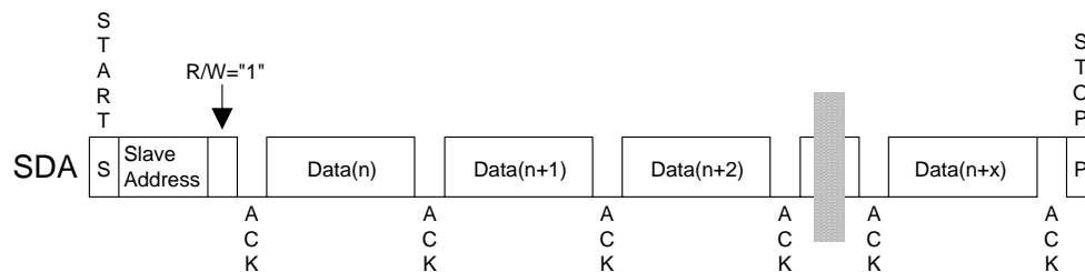
Figure 63. CURRENT ADDRESS READ
