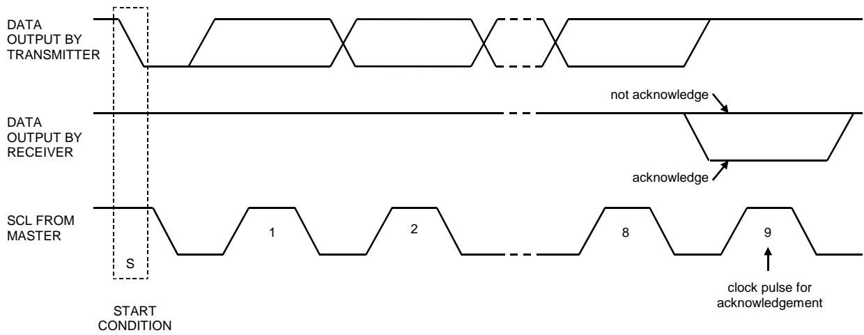
Figure 66. Acknowledge on the I 2 C-Bus
