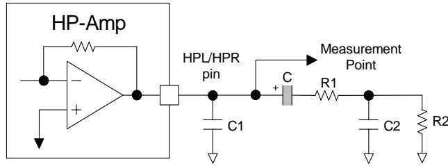
Figure 5. HP-Amp Output Circuit in single-ended mode
