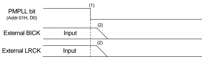
Figure 79. Clock Stopping Sequence (2)
