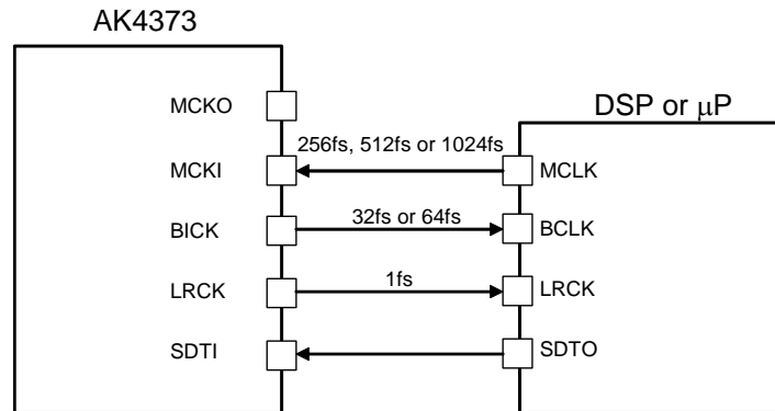
Figure 29. EXT Master Mode
