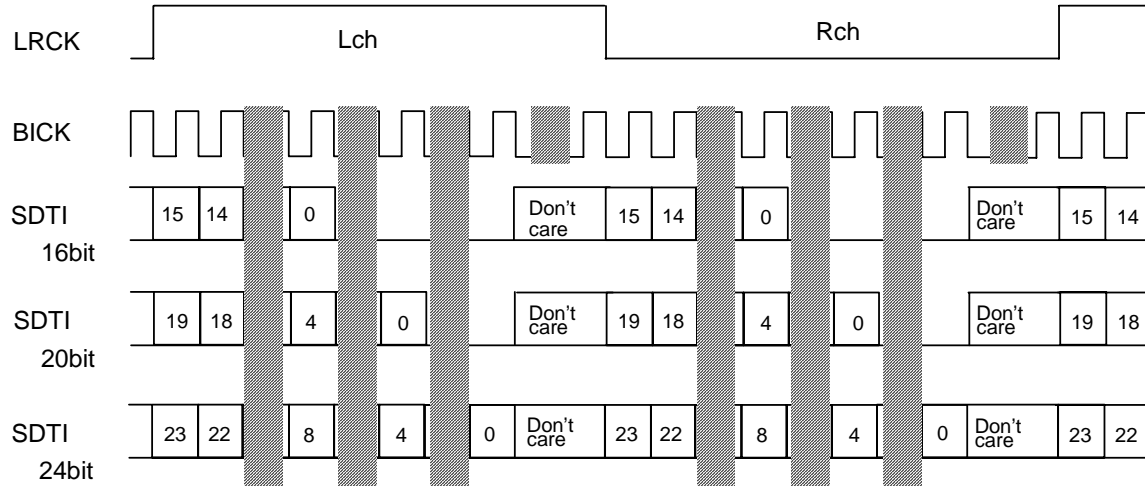
Figure 36. Mode 2 Timing
