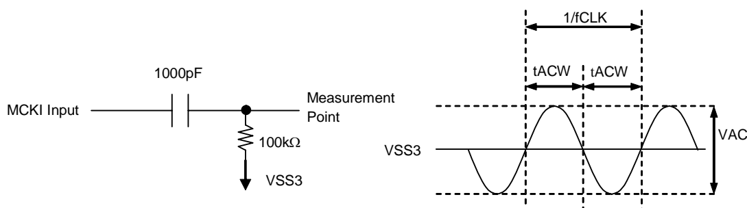
Figure 8. MCKI AC Coupling Timing
