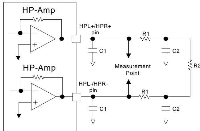
Figure 6. HP-Amp Output Circuit in differential mode
