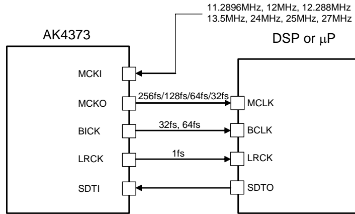
Figure 24. PLL Master Mode
