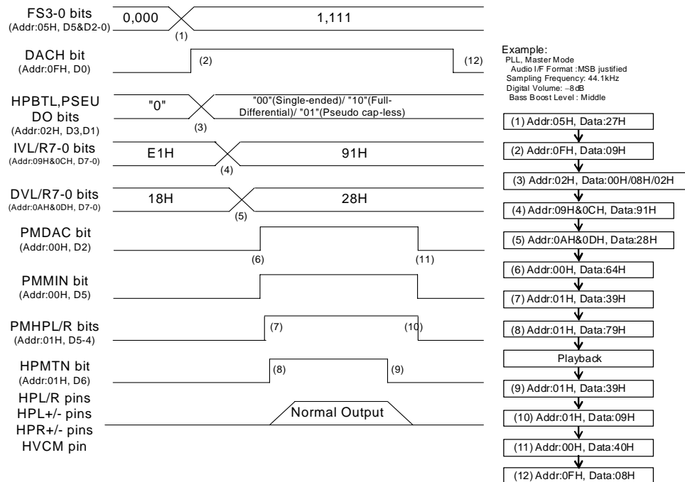
Figure 77. Headphone-Amp Output Sequence
