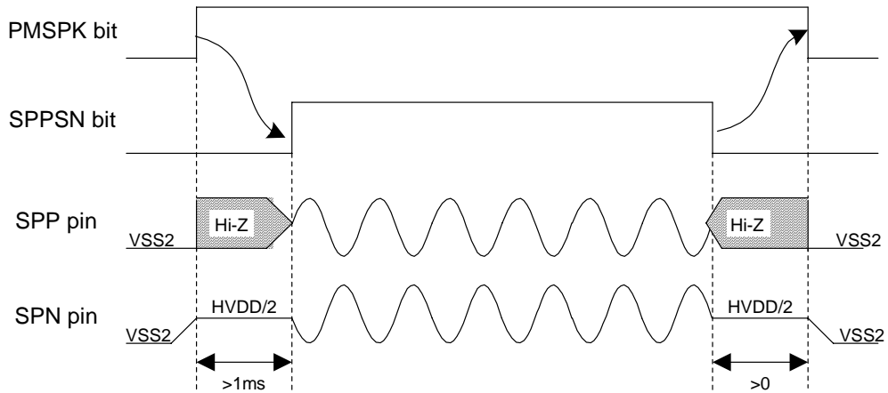
Figure 57. Power-up/Power-down Timing for Speaker-Amp
