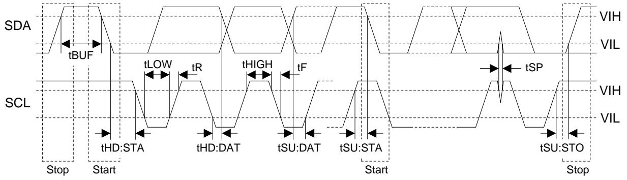
Figure 22. I 2 C Bus Mode Timing
