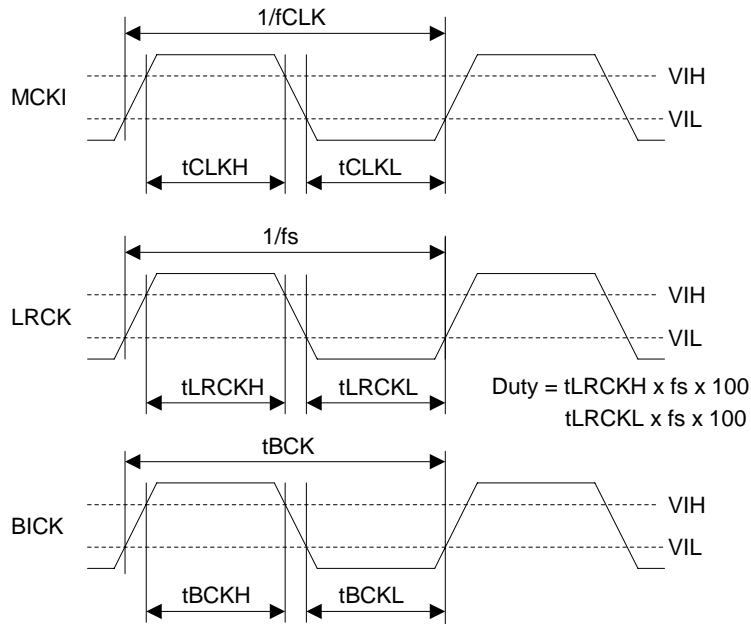
Figure 18. Clock Timing (EXT Slave mode)
