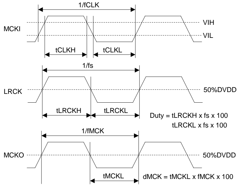
Figure 9. Clock Timing (PLL/EXT Master mode)
