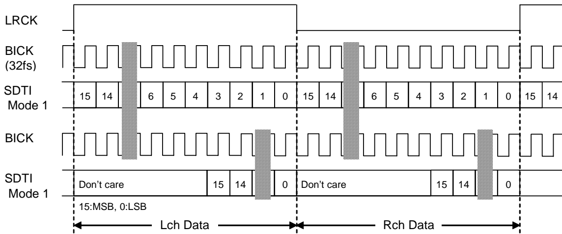
Figure 34. Mode 1 Timing
