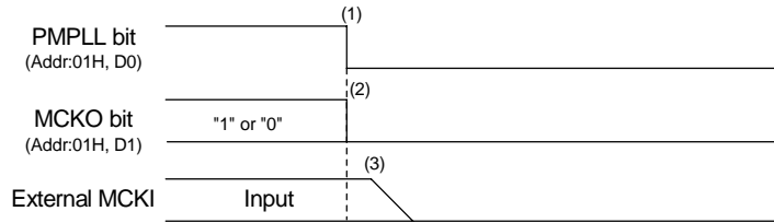
Figure 78. Clock Stopping Sequence (1)
