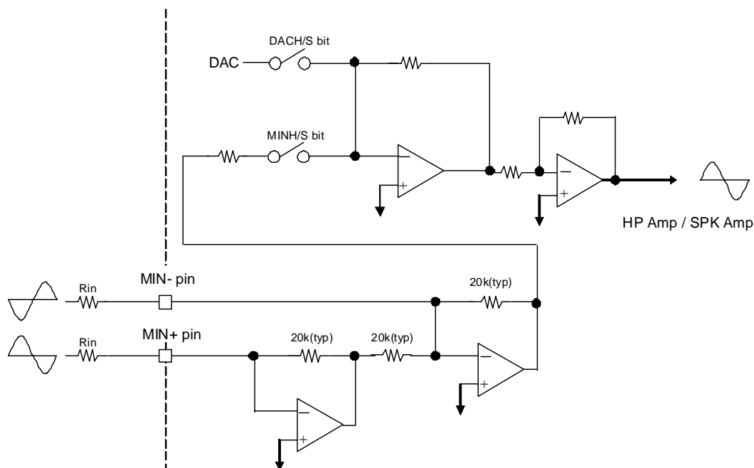
Figure 50. Block Diagram of Monaural input (Differential Input)
