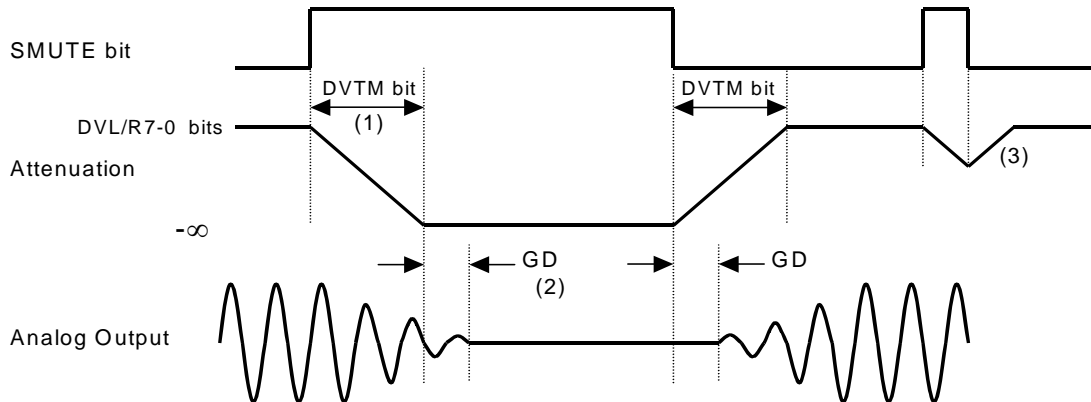
Figure 49. Soft Mute Function
