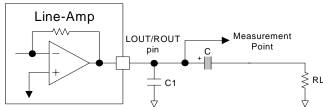
Figure 4. Line-Amp output circuit
