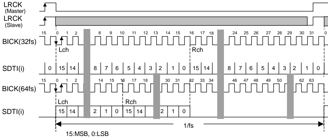
Figure 33. Mode 0 Timing (BCKP = "1", MSBS = "1")
