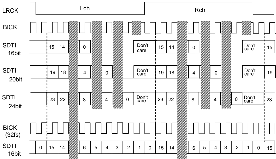
Figure 37. Mode 3 Timing
