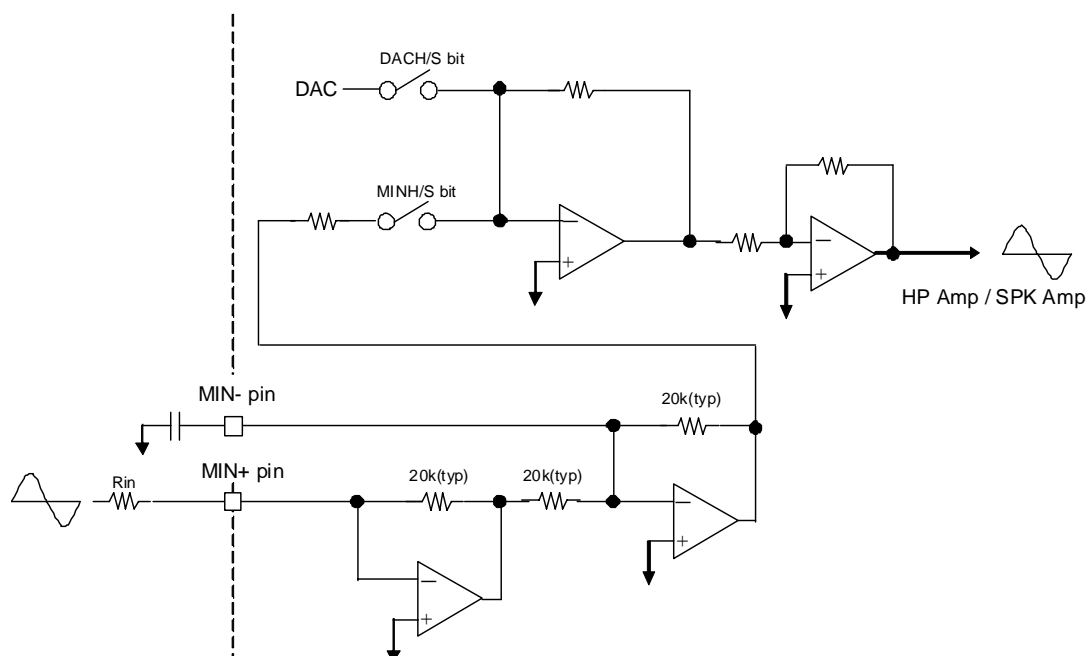
Figure 51. Block Diagram of Monaural input (Single Input)
