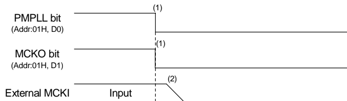
Figure 80. Clock Stopping Sequence (3)
