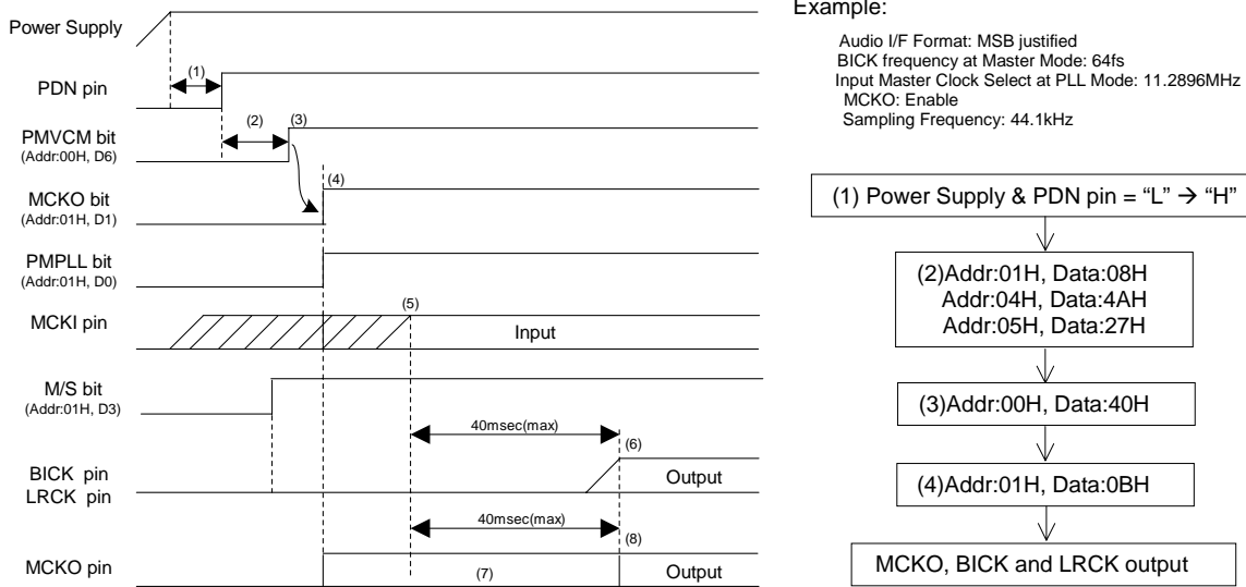
Figure 71. Clock Set Up Sequence (1)
