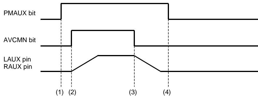
Figure 19. Power-up/Power-down Timing for Aux-out amplifier
