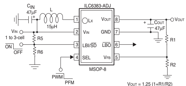
Figure 2. ILC6383CIR-ADJ
