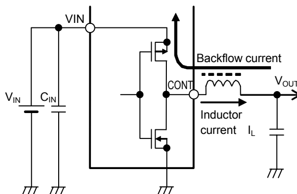
Figure 10 Backflow Current
