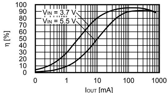
(1) Output current ( I_{OUT} ) vs. Efficiency ( \eta )
