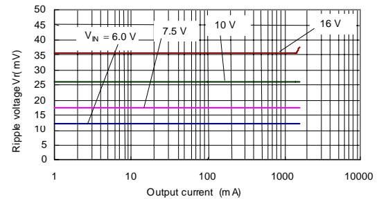
(34) S-8533A50AFT (Si3454DV/Si3455DV)
