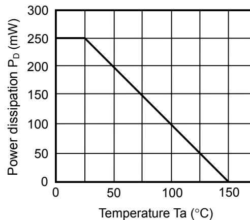
Figure 4 Power Dissipation of Package
