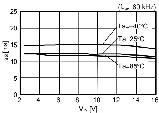
(5) Soft start time ( t_{SS} )-Input voltage ( V_{IN} )
