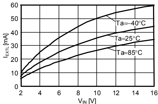
(3) EXT pin output current "H" ( I_{EXTH} )-Input voltage ( V_{IN} ) (4) EXT pin output current "L" ( I_{EXTL} )-Input voltage ( V_{IN} )
