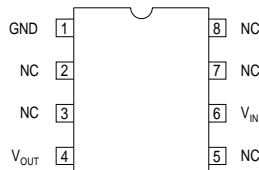
8 Pin J Package
