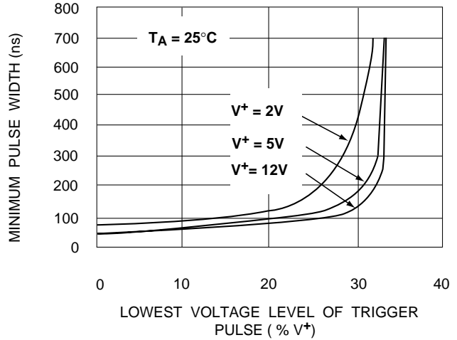
MINIMUM PULSE WIDTH REQUIRED FOR TRIGGERING
