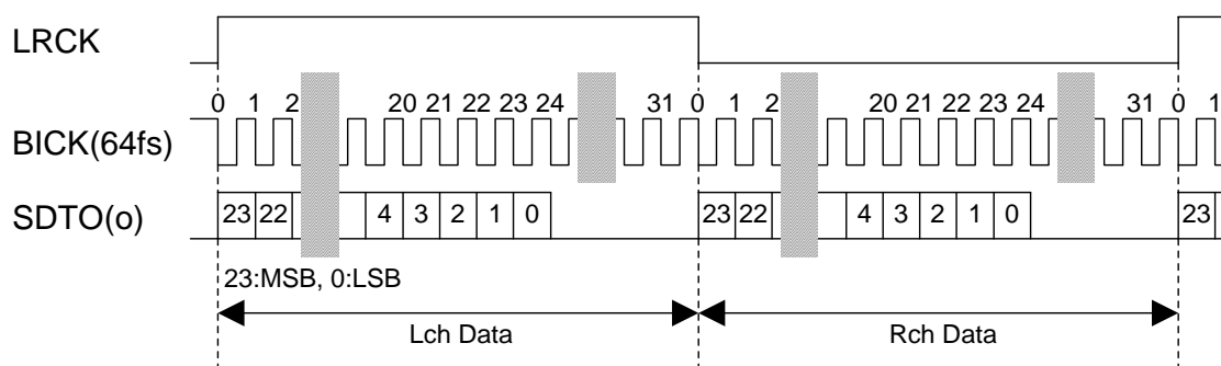
Figure 3. Mode 0 Timing
