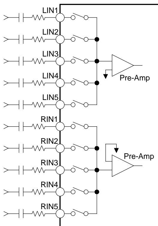
Figure 6. Input Selector
