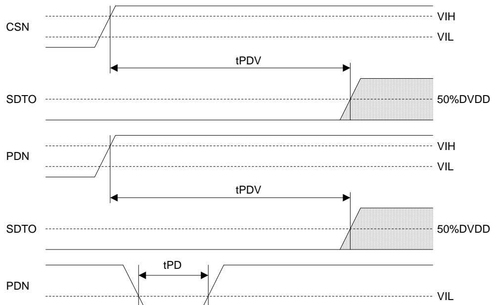
Power Down &amp; Reset Timing
