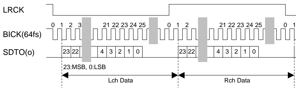
Figure 4. Mode 1 Timing
