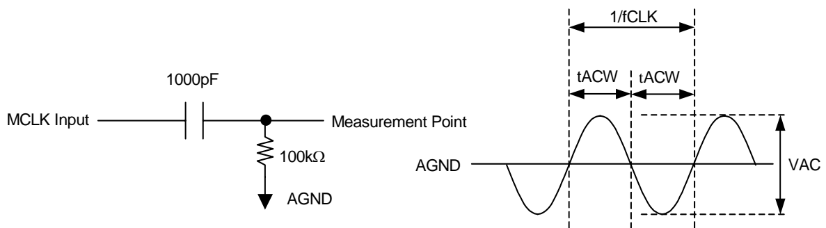
MCLK AC Coupling Timing (Measurement condition)
